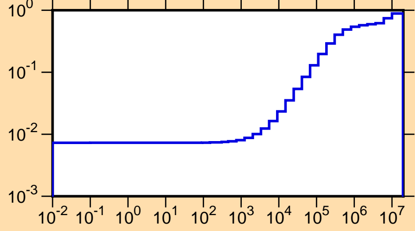
\mu vs. E for ^{96}\text{Rh}(\text{mt251})
