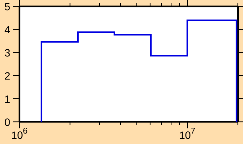
\Delta\sigma/\sigma vs. E for ^{96}\text{Rh}(n,tot.)
