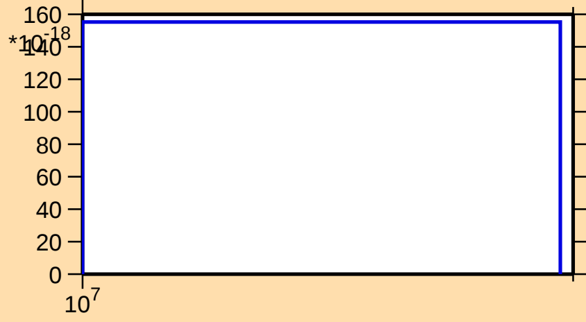
\sigma vs. E for ^{96}\text{Rh}(n,\text{nt})
