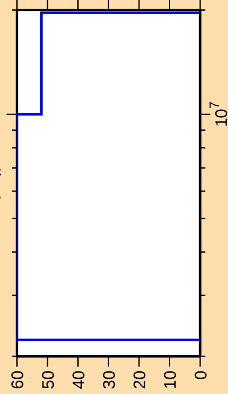
\Delta\sigma/\sigma vs. E for ^{96}\text{Rh}(n,\gamma)
