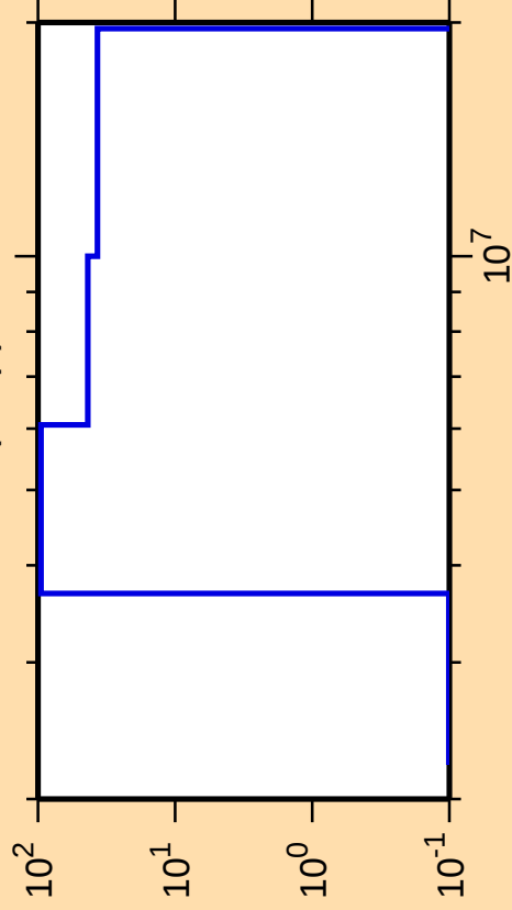
\Delta\sigma/\sigma vs. E for ^{96}\text{Rh}(n,np)
