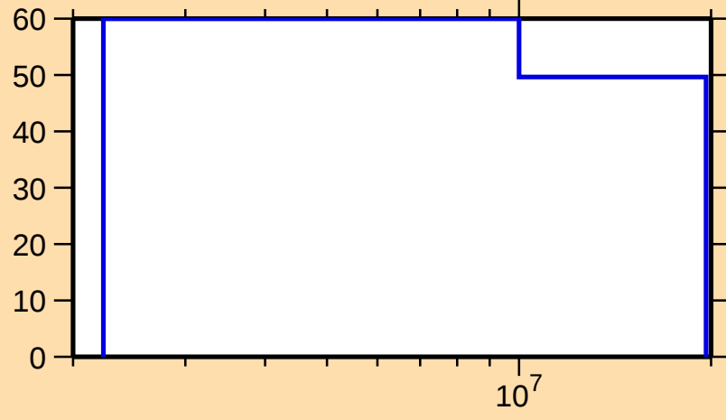
\Delta\sigma/\sigma vs. E for ^{96}\text{Rh}(n,\text{ncont.})
