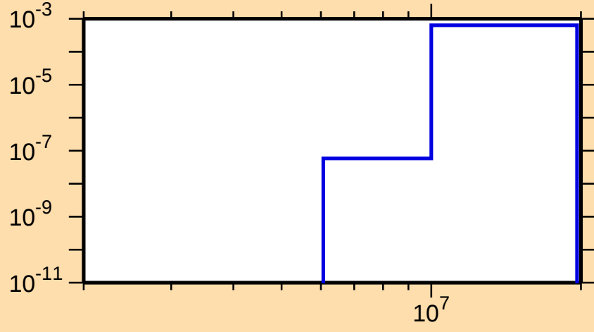
\sigma vs. E for ^{96}\text{Rh}(n,t)
