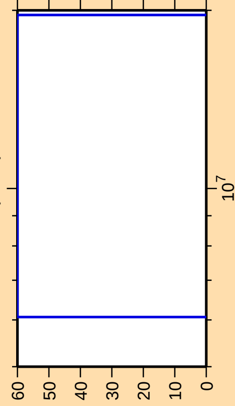
\Delta\sigma/\sigma vs. E for ^{96}\text{Rh}(n,n\alpha)
