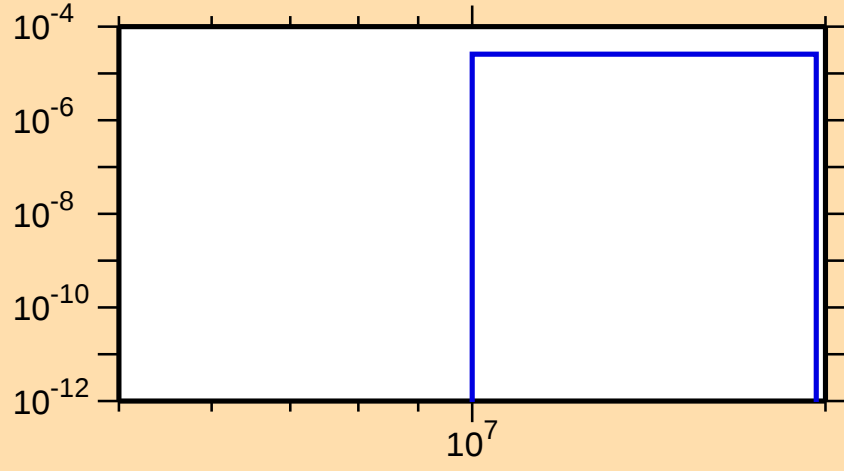
\sigma vs. E for ^{96}\text{Rh}(n,\text{pd})
