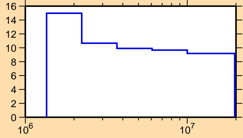
\Delta\sigma/\sigma vs. E for ^{97}\text{Rh}(n,n\text{onrel.})
