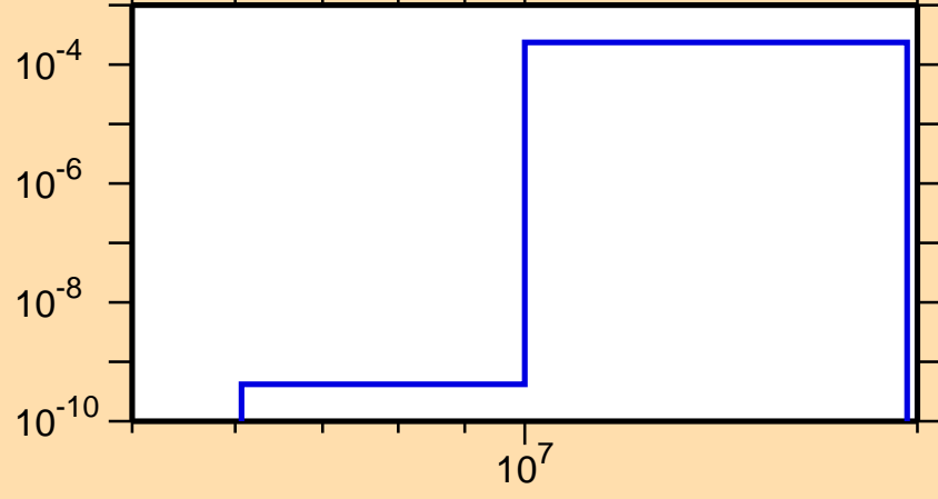
\sigma vs. E for ^{97}\text{Rh}(n,t)
