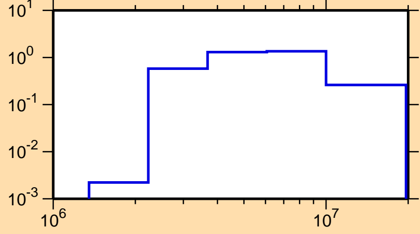
\sigma vs. E for ^{97}\text{Rh}(n,n\text{cont.})
