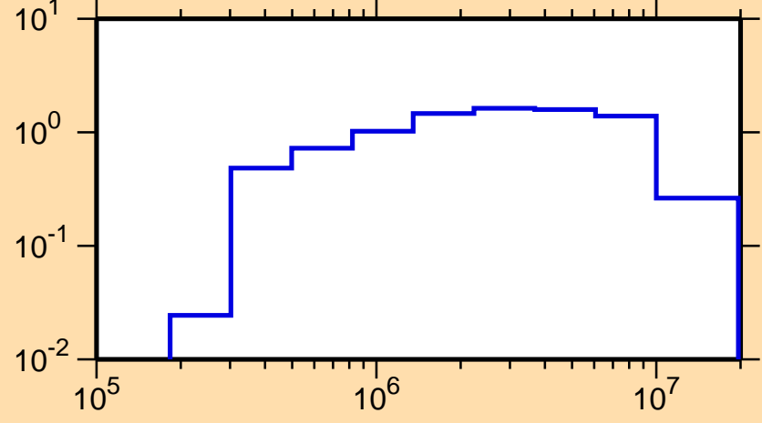
\sigma vs. E for ^{97}\text{Rh}(n,\text{inel.})
