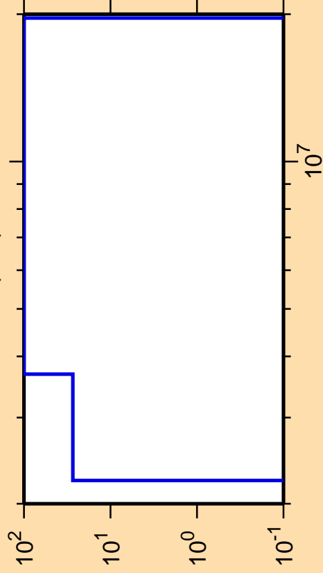
\Delta\sigma/\sigma vs. E for ^{97}\text{Rh}(n,d)
