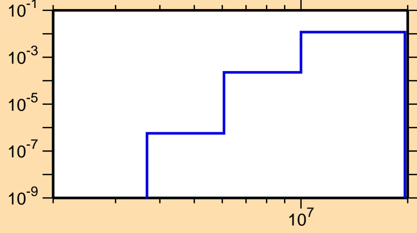
\sigma vs. E for ^{97}\text{Rh}(n,d)
