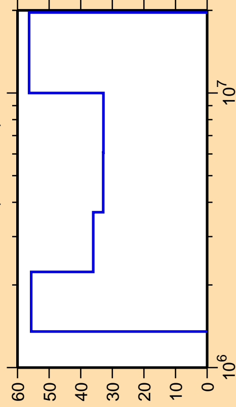
\Delta\sigma/\sigma vs. E for ^{97}\text{Rh}(n,\text{ncont.})
