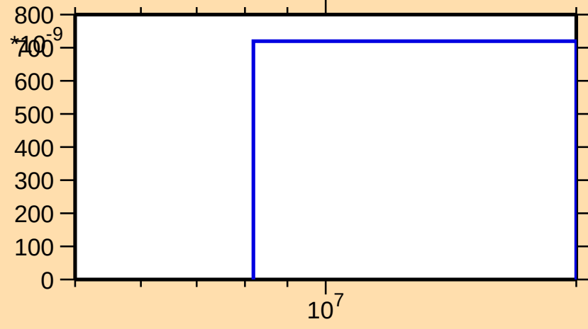
\sigma vs. E for ^{97}\text{Rh}(n,\text{pd})
