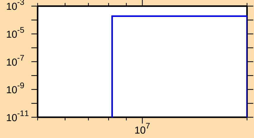
\sigma vs. E for ^{97}\text{Rh}(n,t)
