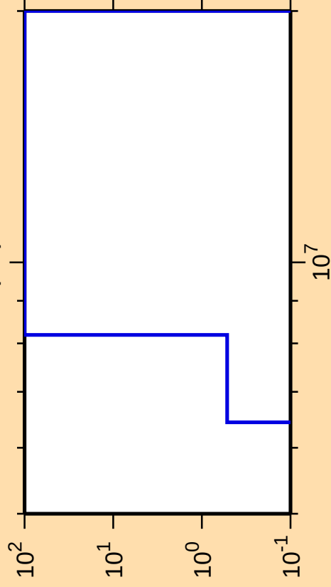
\Delta\sigma/\sigma vs. E for ^{97}\text{Rh}(n,t)
