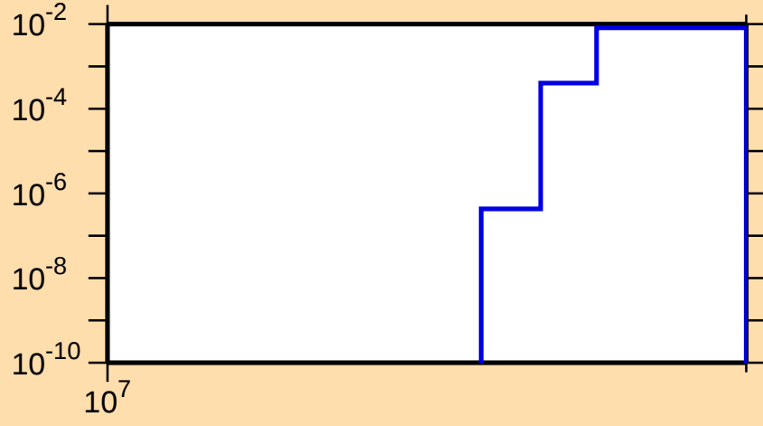
\sigma vs. E for ^{97}\text{Rh}(n,2np)
