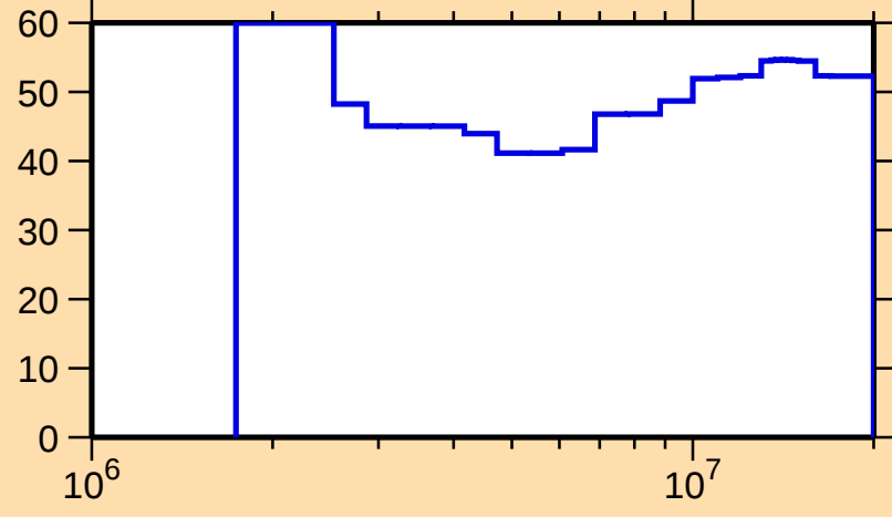
\Delta\sigma/\sigma vs. E for ^{97}\text{Rh}(n,ncont.)
