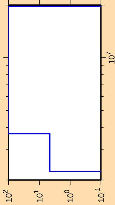
\Delta\sigma/\sigma vs. E for ^{97}\text{Rh}(n,p\alpha)
