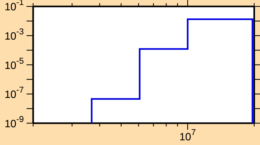
\sigma vs. E for ^{97}\text{Rh}(n,p\alpha)
