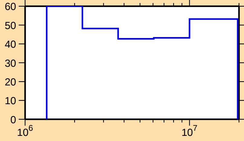
\Delta\sigma/\sigma vs. E for ^{97}\text{Rh}(n,n\text{cont.})
