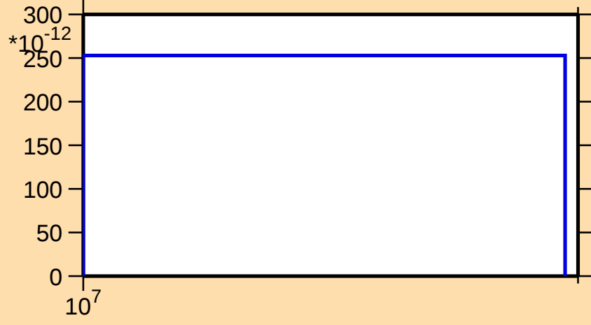
\sigma vs. E for ^{97}\text{Rh}(n,\text{nt})
