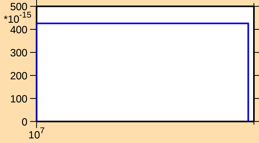
\sigma vs. E for ^{97}\text{Rh}(\text{mt } 34)
