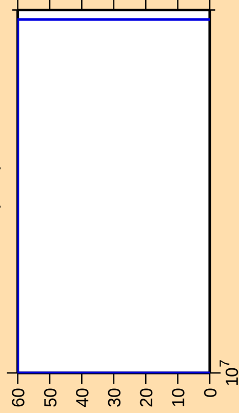
\Delta\sigma/\sigma vs. E for ^{97}\text{Rh}(n,\text{nt})
