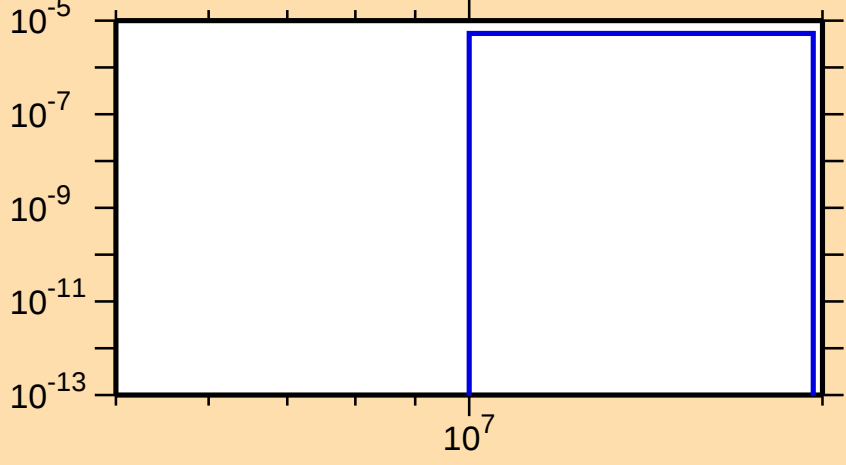
\sigma vs. E for ^{97}\text{Rh}(\text{mt } 45)
