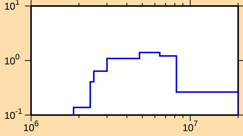
\sigma vs. E for ^{97}\text{Rh}(n,n\text{cont.})
