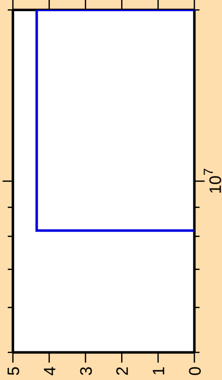
\Delta\sigma/\sigma vs. E for ^{97}\text{Rh}(\text{mt } 34)
