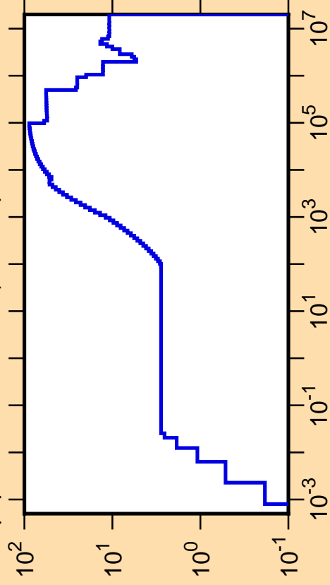
\Delta\mu/\mu vs. E for ^{99}\text{Rh}(\text{mt251})
