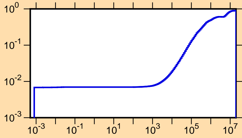
\mu vs. E for ^{99}\text{Rh}(\text{mt251})
