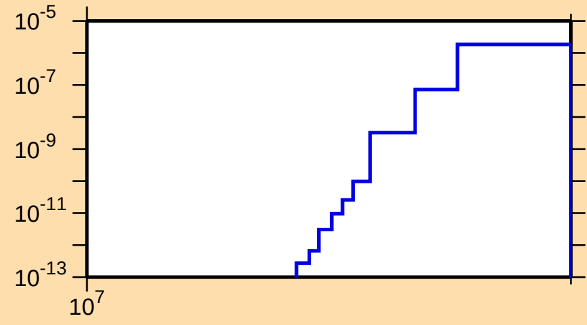
\sigma vs. E for ^{99}\text{Rh}(\text{mt } 45)
