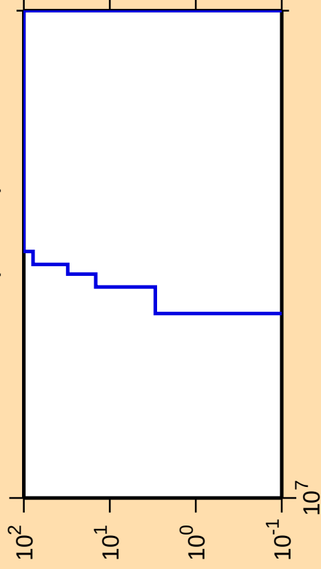
\Delta\sigma/\sigma vs. E for ^{99}\text{Rh(mt117)}
