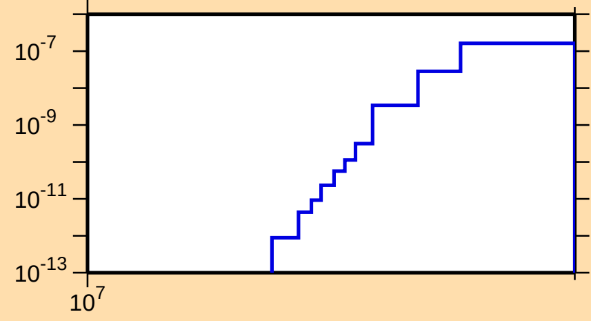
\sigma vs. E for ^{99}\text{Rh(mt117)}
