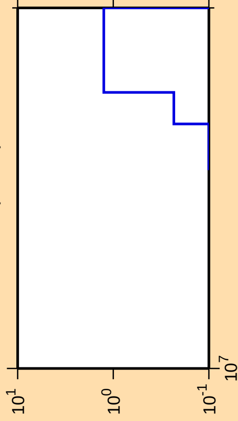
\Delta\sigma/\sigma vs. E for ^{99}\text{Rh}(\text{mt } 34)
