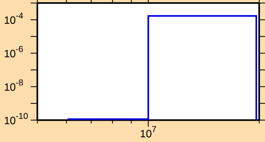
\sigma vs. E for ^{99}\text{Rh}(n,t)
