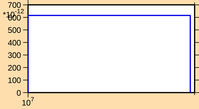
\sigma vs. E for ^{99}\text{Rh}(n,\text{nt})
