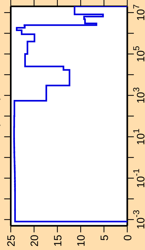
\Delta\sigma/\sigma vs. E for ^{99}\text{Rh}(n,\text{el.})
