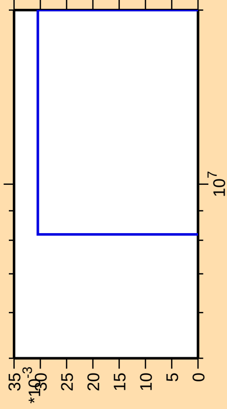
\Delta\sigma/\sigma vs. E for ^{99}\text{Rh}(\text{mt } 34)
