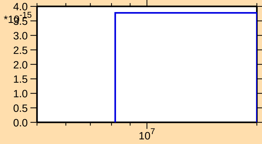
\sigma vs. E for ^{99}\text{Rh}(\text{mt } 34)
