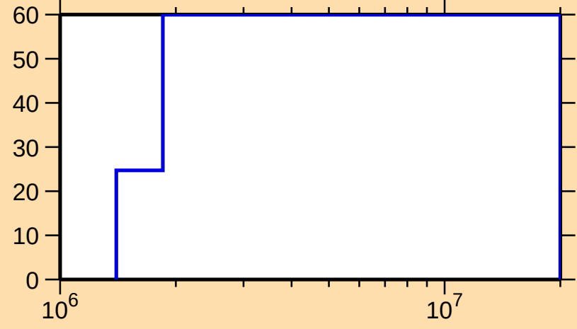
\Delta\sigma/\sigma vs. E for ^{99}\text{Rh}(n,n_1)
