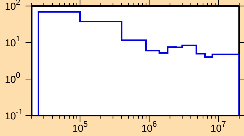
\Delta\sigma/\sigma vs. E for ^{99}\text{Rh}(n,\text{nonel.})
