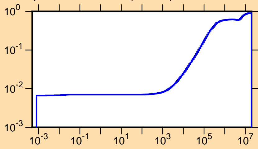
\mu vs. E for ^{102}\text{Rh}(\text{mt251})
