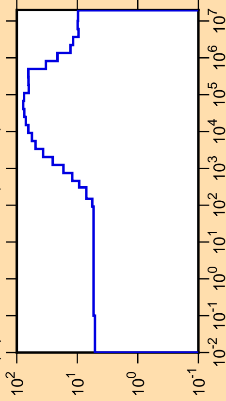
\Delta\mu/\mu vs. E for ^{102}\text{Rh}(\text{mt251})
