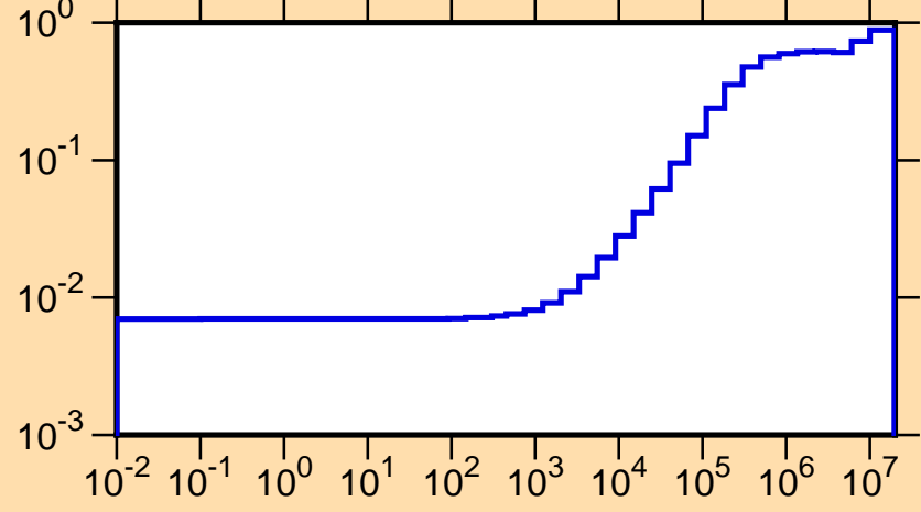
\mu vs. E for ^{102}\text{Rh}(\text{mt251})
