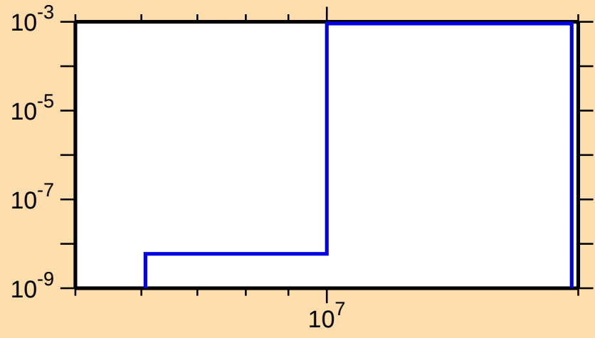
\sigma vs. E for ^{103}\text{Rh}(n,\alpha)
