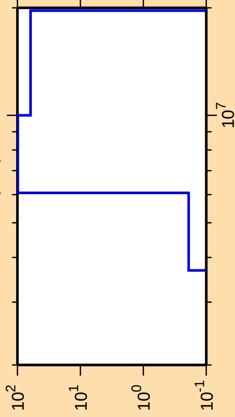
\Delta\sigma/\sigma vs. E for ^{103}\text{Rh}(n,d)
