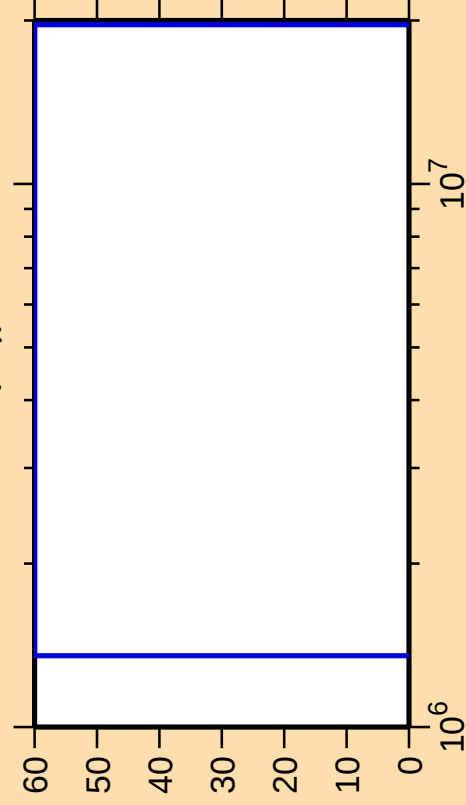
\Delta\sigma/\sigma vs. E for ^{103}\text{Rh}(n,\gamma)
