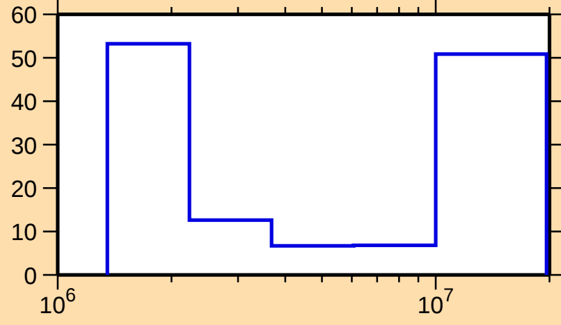
\Delta\sigma/\sigma vs. E for ^{103}\text{Rh}(n,\text{ncont.})
