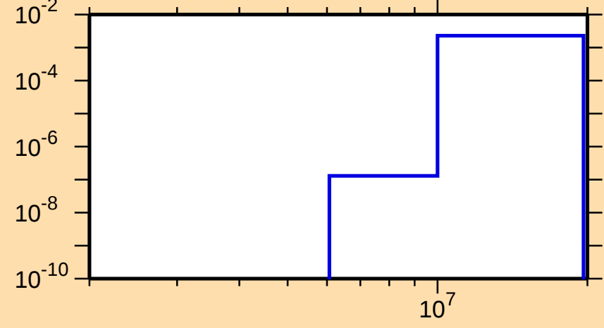
\sigma vs. E for ^{103}\text{Rh}(n,d)
