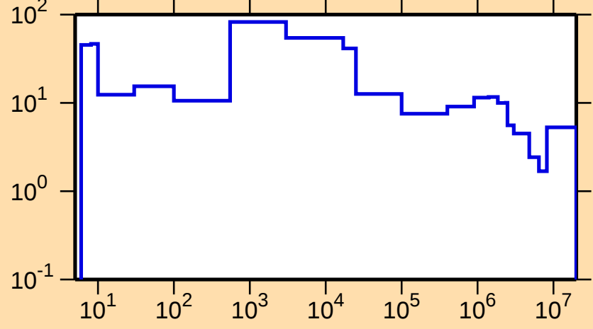
\Delta\sigma/\sigma vs. E for ^{103}\text{Rh}(n,\text{tot.})
