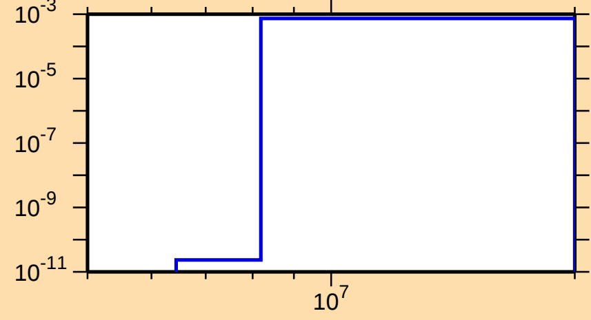
\sigma vs. E for ^{103}\text{Rh}(n,\alpha)
