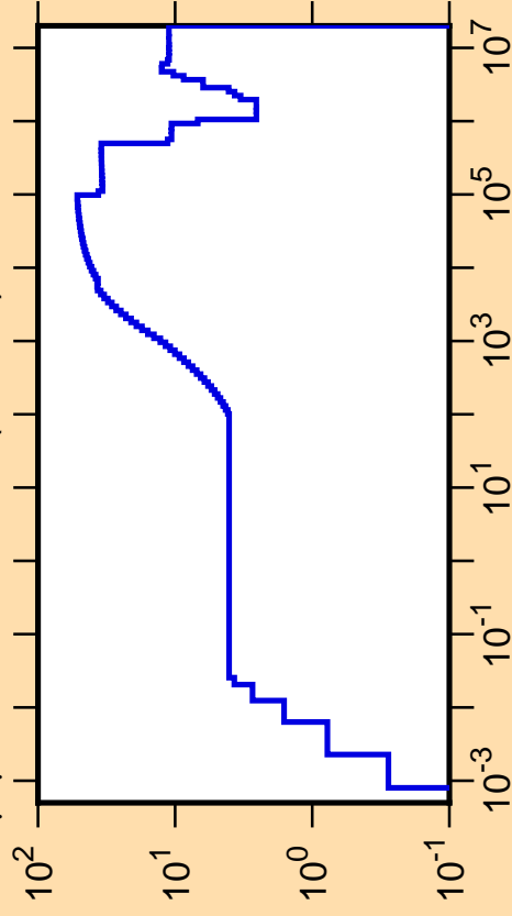
\Delta\mu/\mu vs. E for ^{104}\text{Rh}(\text{mt251})
