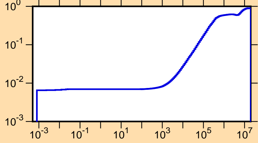
\mu vs. E for ^{104}\text{Rh}(\text{mt251})
