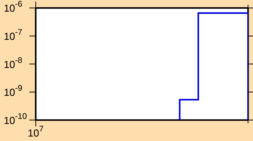
\sigma vs. E for ^{104}\text{Rh}(n,\text{nt})
