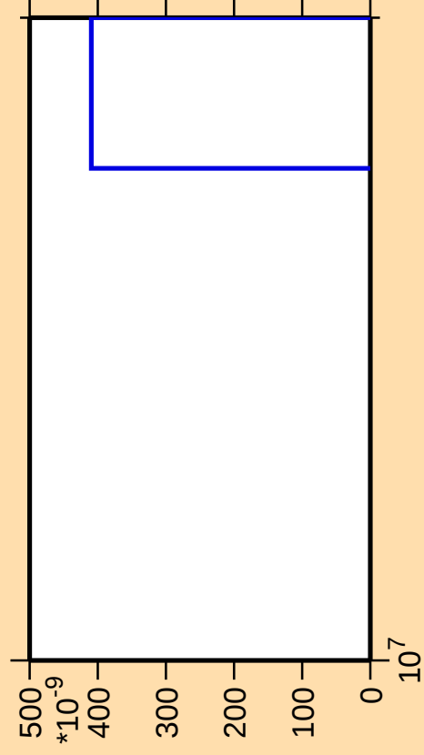
\Delta\sigma/\sigma vs. E for ^{104}\text{Rh}(n,3n\alpha)
