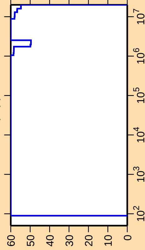
\Delta\sigma/\sigma vs. E for ^{104}\text{Rh}(n,p)
