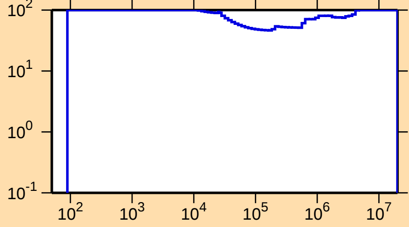
\Delta\sigma/\sigma vs. E for ^{104}\text{Rh}(n,n_1)
