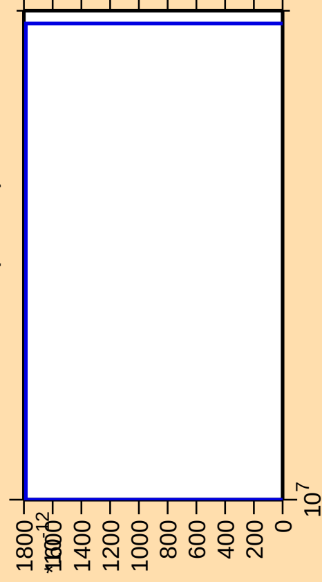
\Delta\sigma/\sigma vs. E for ^{104}\text{Rh}(n,3n\alpha)
