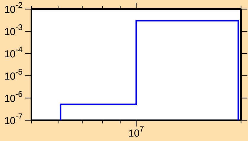
\sigma vs. E for ^{104}\text{Rh}(n,d)
