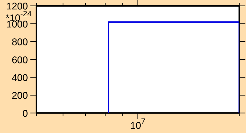
\sigma vs. E for ^{104}\text{Rh}(n,3n\alpha)
