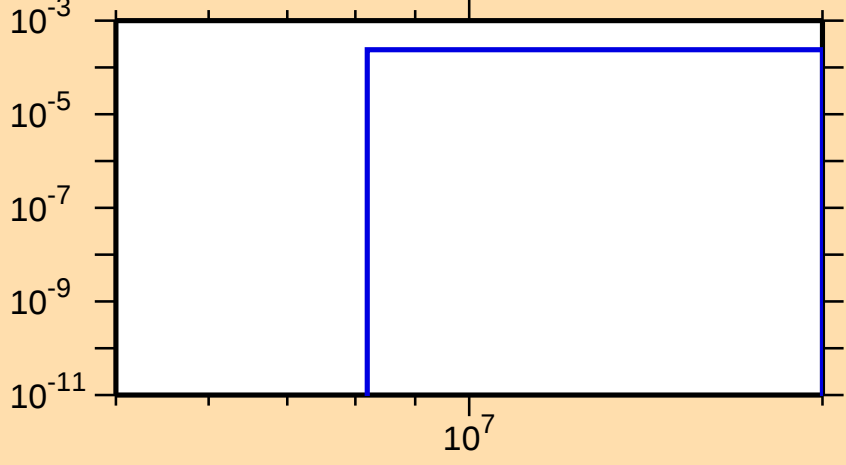
\sigma vs. E for ^{104}\text{Rh}(n,t)
