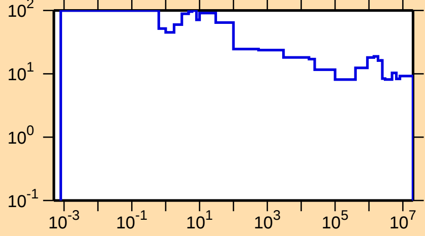
\Delta\sigma/\sigma vs. E for ^{104}\text{Rh}(n,\text{el.})
