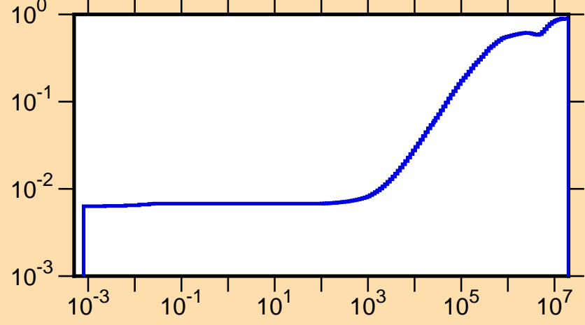
\mu vs. E for ^{107}\text{Rh}(\text{mt251})
