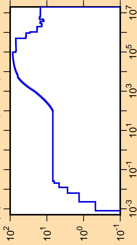
\Delta\mu/\mu vs. E for ^{107}\text{Rh}(\text{mt251})
