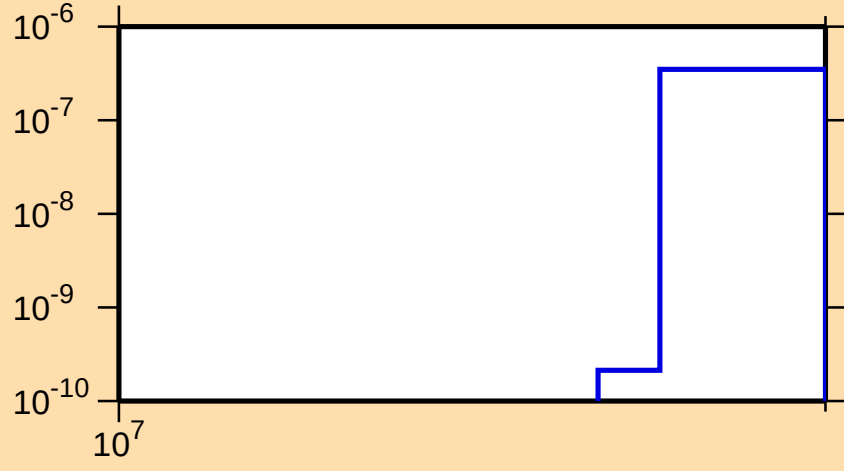
\sigma vs. E for ^{107}\text{Rh}(n,\text{nt})
