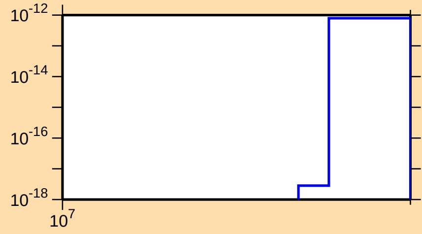
\sigma vs. E for ^{107}\text{Rh}(n,\text{He3})
