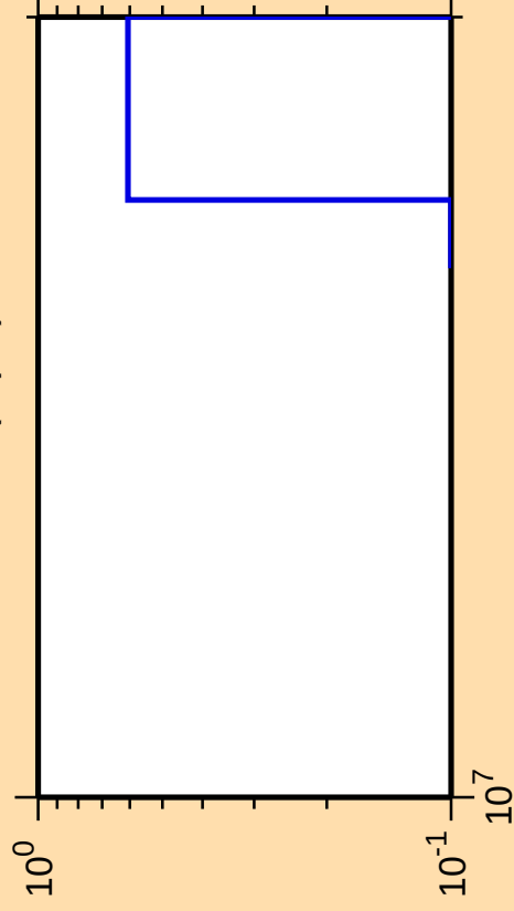
\Delta\sigma/\sigma vs. E for ^{107}\text{Rh}(n,p\alpha)
