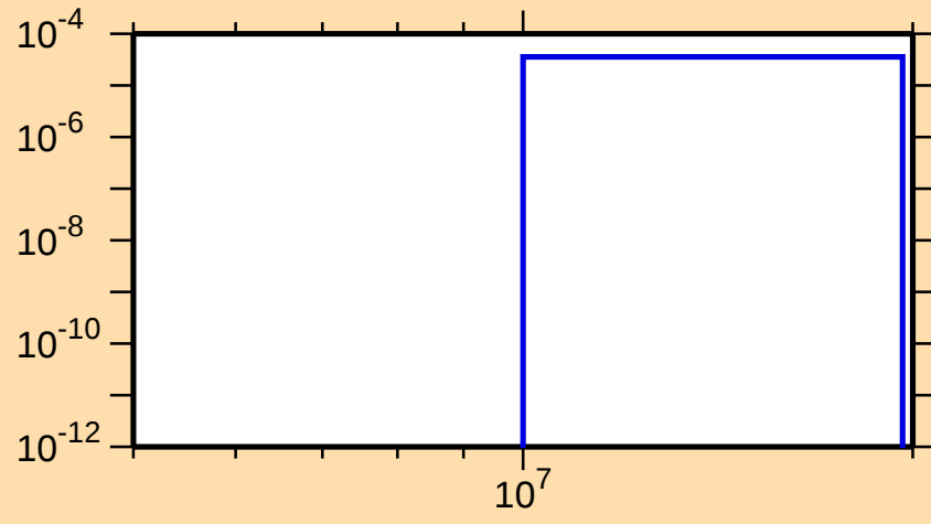
\sigma vs. E for ^{107}\text{Rh}(n,\alpha)
