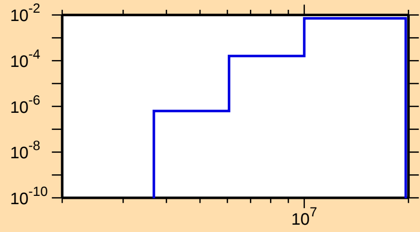
\sigma vs. E for ^{107}\text{Rh}(n,p)
