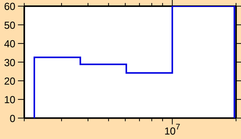
\Delta\sigma/\sigma vs. E for ^{107}\text{Rh}(n,n\text{cont.})
