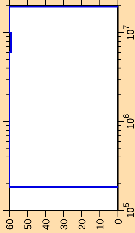
\Delta\sigma/\sigma vs. E for ^{107}\text{Rh}(n,\gamma)
