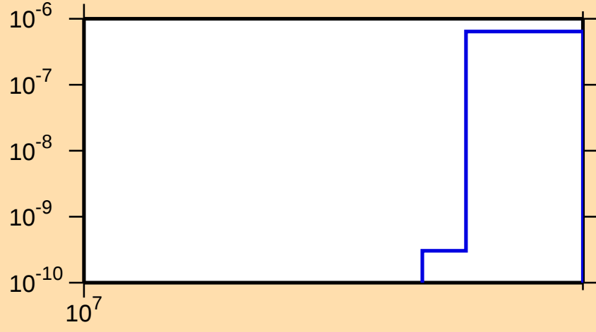
\sigma vs. E for ^{108}\text{Rh}(n,\text{nt})
