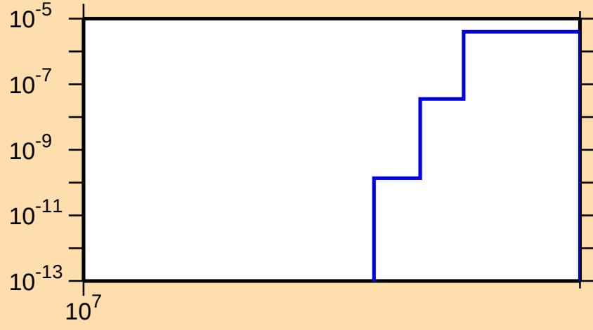
\sigma vs. E for ^{108}\text{Rh}(n,2np)
