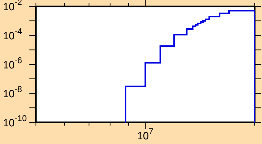
\sigma vs. E for ^{108}\text{Rh}(n,d)
