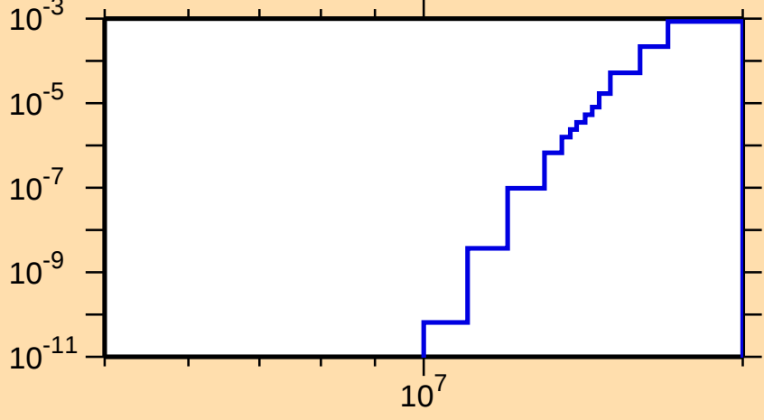
\sigma vs. E for ^{108}\text{Rh}(n,\alpha)
