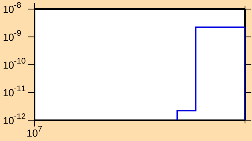
\sigma vs. E for ^{112}\text{Rh}(n,2n\alpha)
