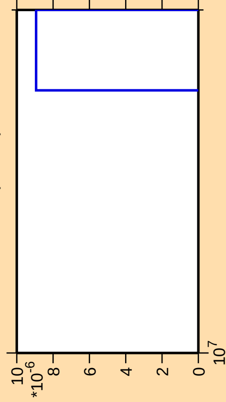
\Delta\sigma/\sigma vs. E for ^{112}\text{Rh}(\text{mt } 11)
