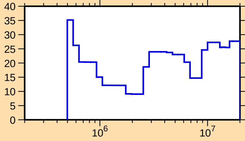
\Delta\sigma/\sigma vs. E for ^{112}\text{Rh}(n,n\text{oncl.})
