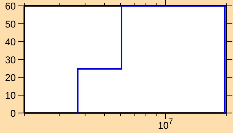
\Delta\sigma/\sigma vs. E for ^{112}\text{Rh}(n,ncont.)
