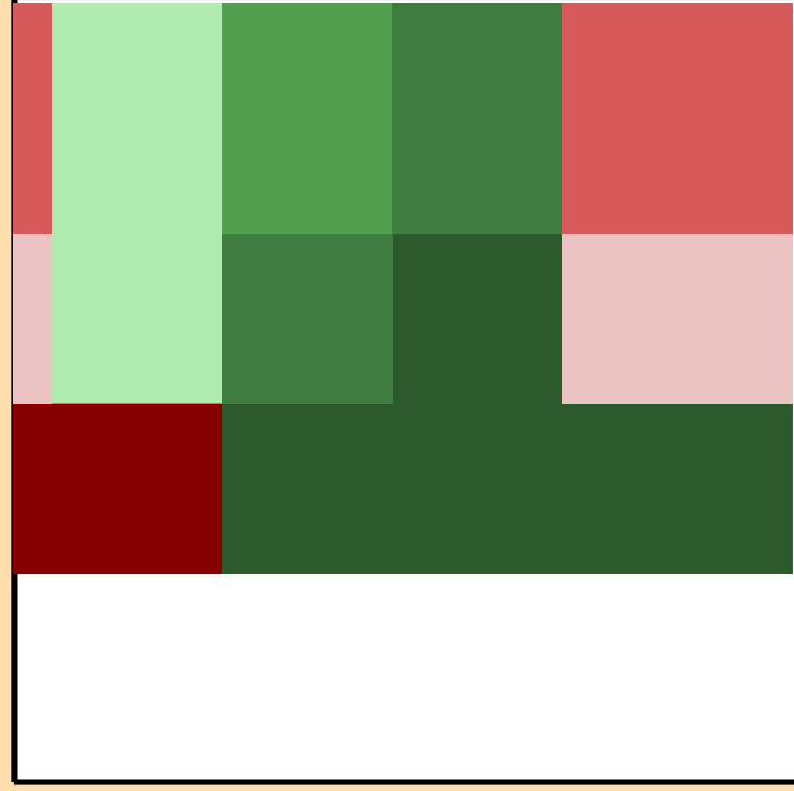
\Delta\sigma/\sigma vs. E for ^{112}\text{Rh}(n,\text{tot.})
