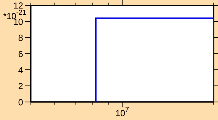
\sigma vs. E for ^{112}\text{Rh}(\text{mt } 11)
