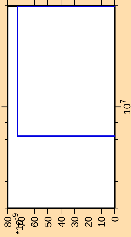
\Delta\sigma/\sigma vs. E for ^{112}\text{Rh}(\text{mt } 11)
