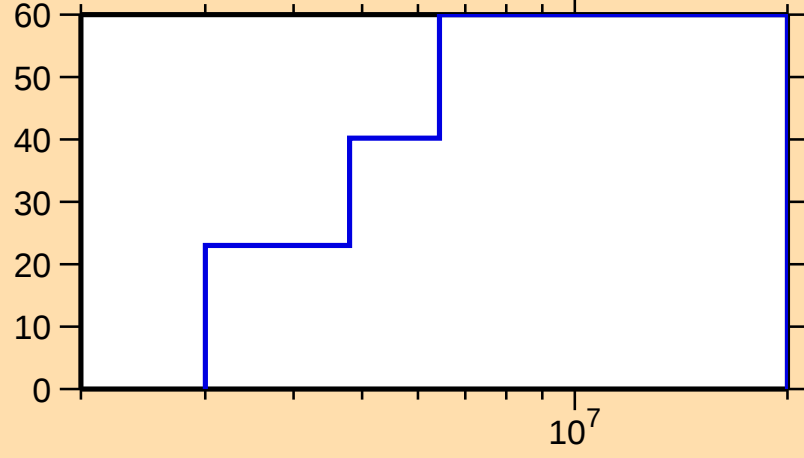
\Delta\sigma/\sigma vs. E for ^{112}\text{Rh}(n,\text{ncont.})
