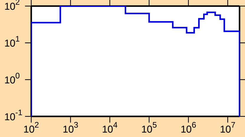
\Delta\sigma/\sigma vs. E for ^{112}\text{Rh}(n,\text{el.})
