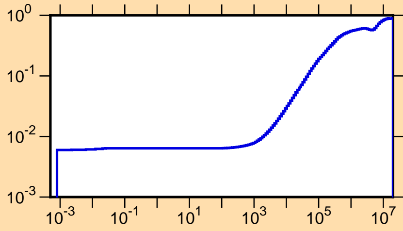
\mu vs. E for ^{113}\text{Rh}(\text{mt251})
