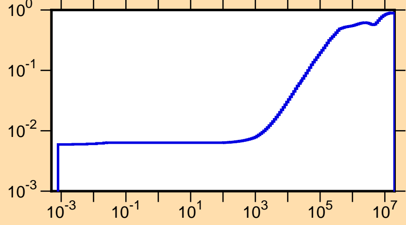
\mu vs. E for ^{114}\text{Rh}(\text{mt251})
