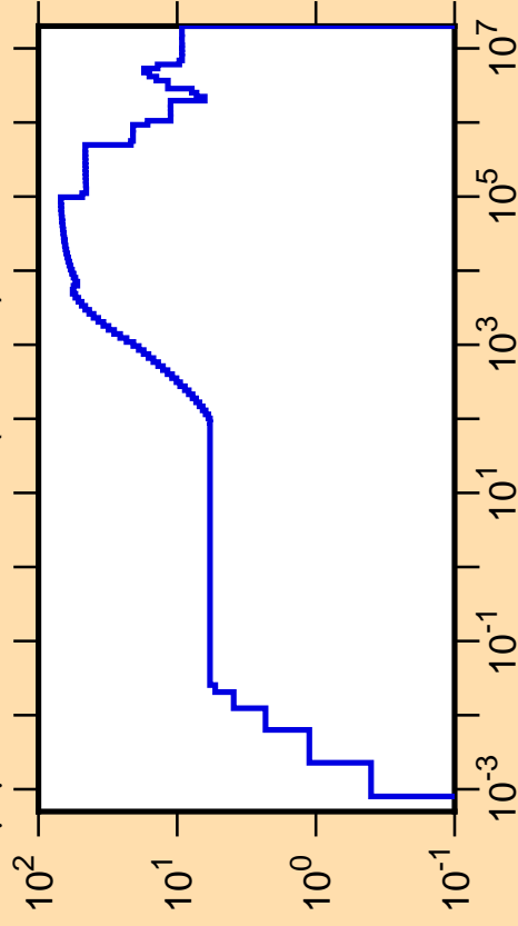
\Delta\mu/\mu vs. E for ^{114}\text{Rh}(\text{mt251})
