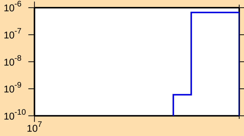
\sigma vs. E for ^{114}\text{Rh}(n,\text{nt})
