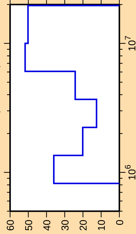
\Delta\sigma/\sigma vs. E for ^{114}\text{Rh}(n,\text{ncont.})
