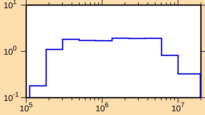
\sigma vs. E for ^{114}\text{Rh}(n,\text{inel.})
