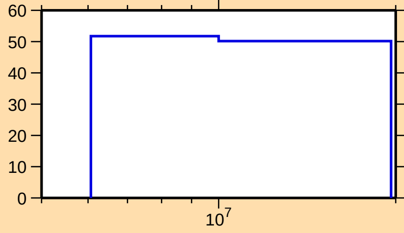
\Delta\sigma/\sigma vs. E for ^{114}\text{Rh}(n,\text{ncont.})
