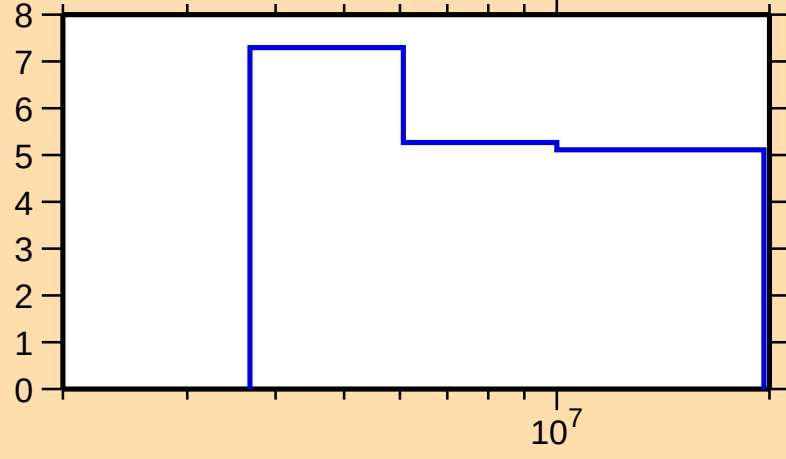
\Delta\sigma/\sigma vs. E for ^{114}\text{Rh}(n,\text{nonel.})
