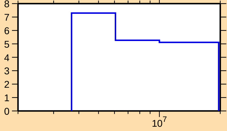
\Delta\sigma/\sigma vs. E for ^{114}\text{Rh}(n,\text{nonel.})
