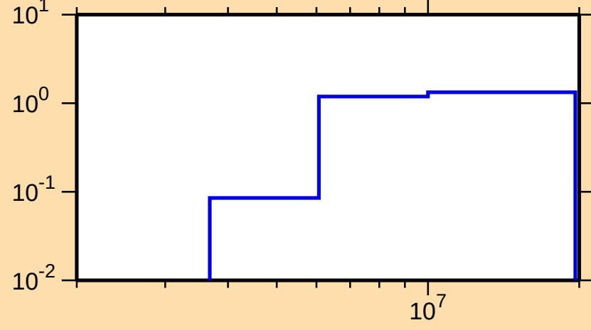
\sigma vs. E for ^{114}\text{Rh}(n,2n)
