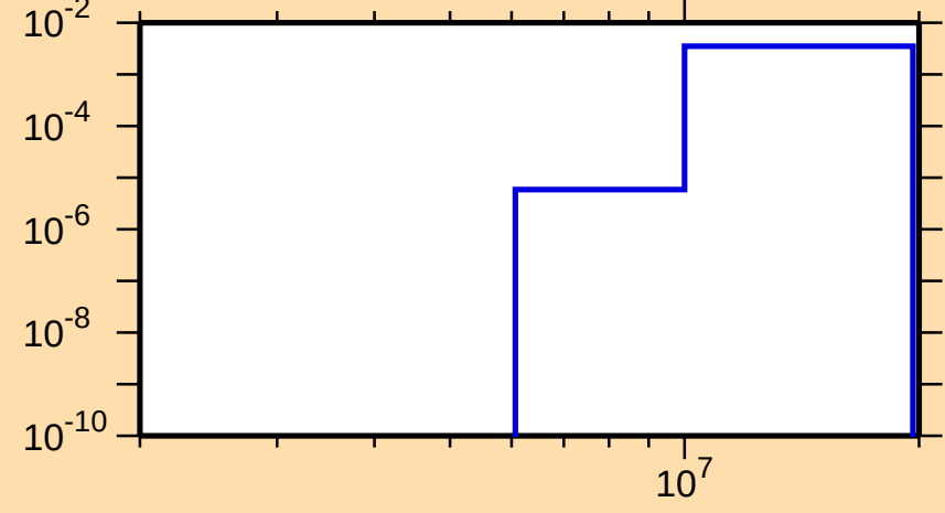
\sigma vs. E for ^{114}\text{Rh}(n,p)
