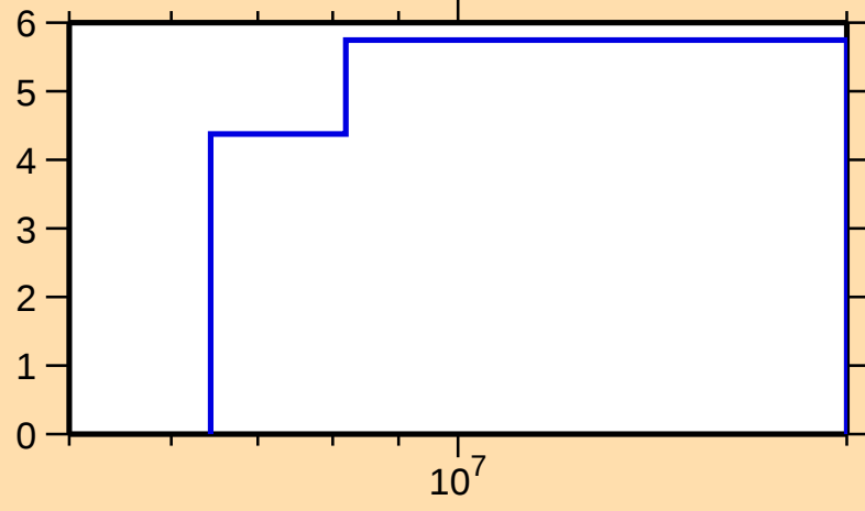
\Delta\sigma/\sigma vs. E for ^{114}\text{Rh}(n,\text{tot.})
