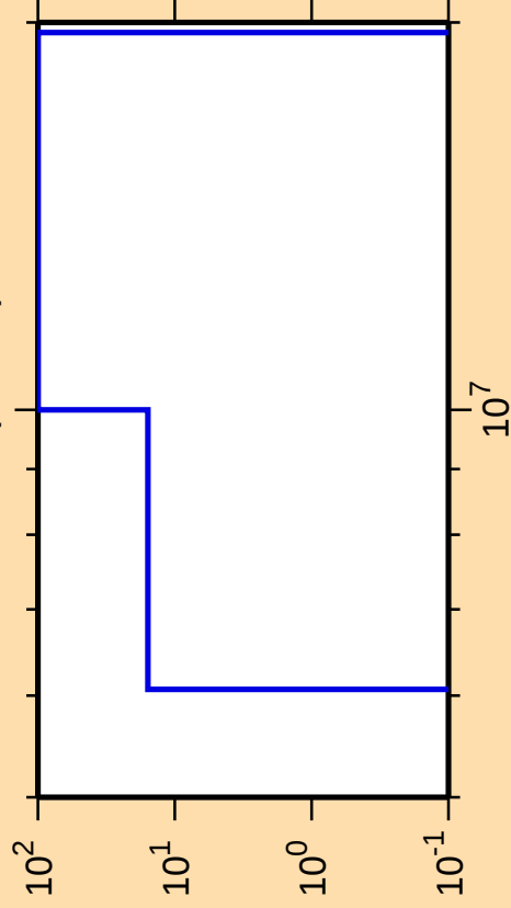
\Delta\sigma/\sigma vs. E for ^{200}\text{Rn}(\text{mt } 45)
