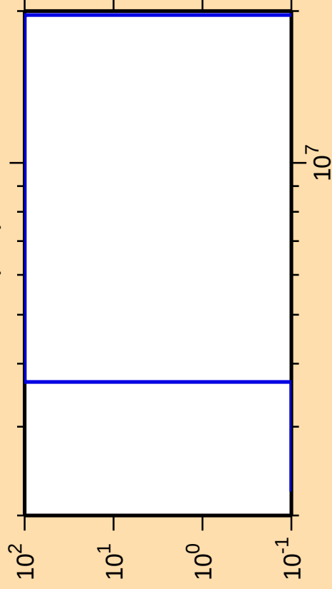
\Delta\sigma/\sigma vs. E for ^{200}\text{Rn}(n,d)
