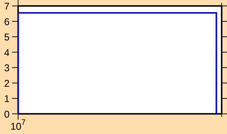
\Delta\sigma/\sigma vs. E for ^{200}\text{Rn}(n,\text{el.})
