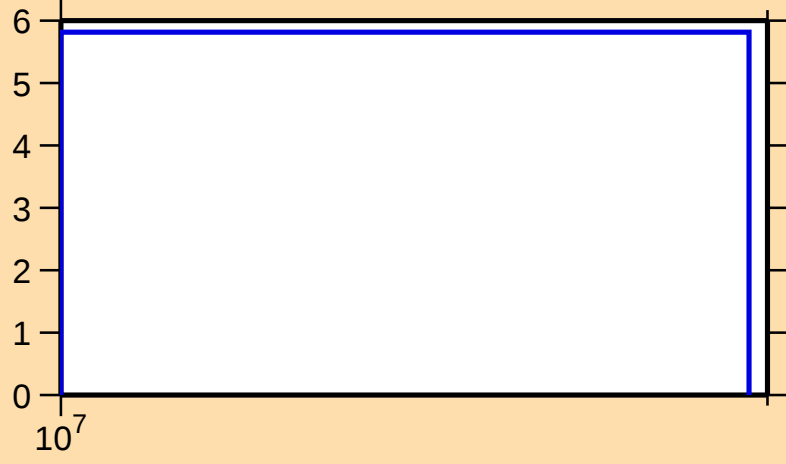
\Delta\sigma/\sigma vs. E for ^{200}\text{Rn}(n,\text{tot.})
