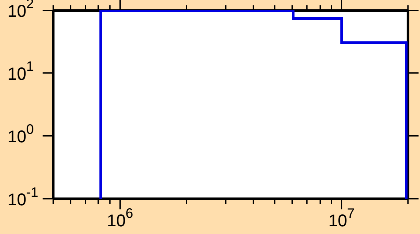
\Delta\sigma/\sigma vs. E for ^{200}\text{Rn}(n,n\text{cont.})
