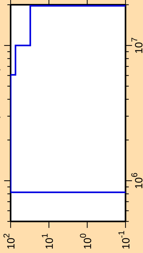
\Delta\sigma/\sigma vs. E for ^{200}\text{Rn}(n,n_{\text{cont}})
