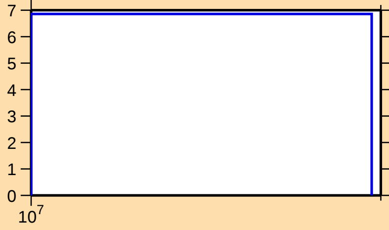
\Delta\sigma/\sigma vs. E for ^{200}\text{Rn}(n,\text{nonel.})
