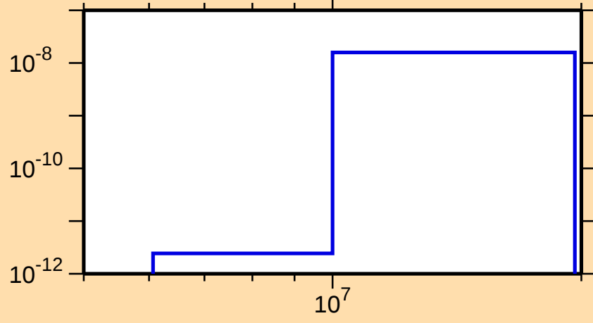
\sigma vs. E for ^{200}\text{Rn}(\text{mt } 45)
