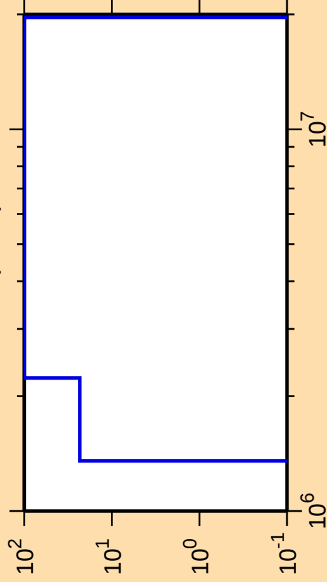
\Delta\sigma/\sigma vs. E for ^{200}\text{Rn}(n,n\alpha)
