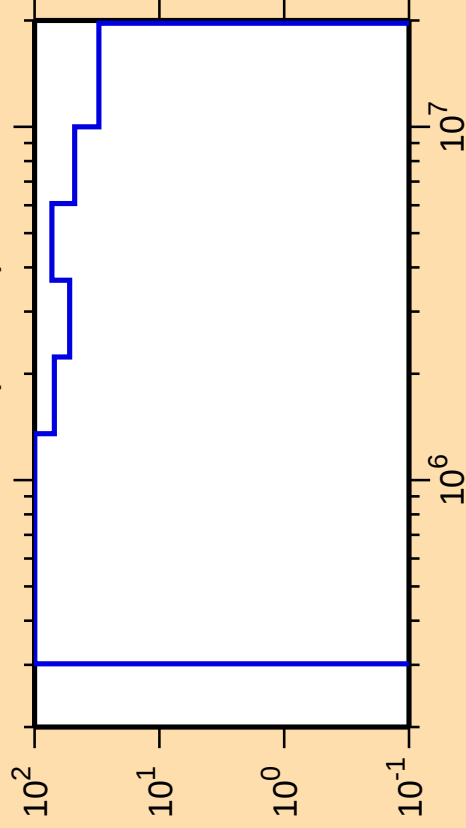
\Delta\sigma/\sigma vs. E for ^{200}\text{Rn}(n,\text{inel.})
