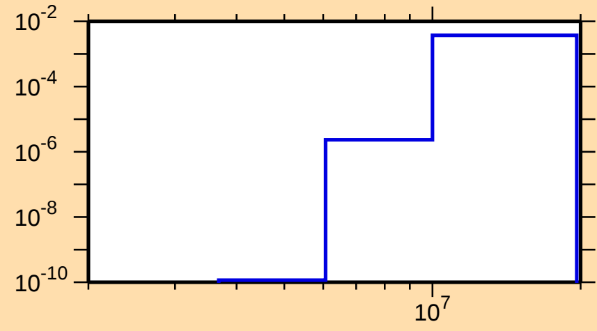
\sigma vs. E for ^{200}\text{Rn}(n,d)
