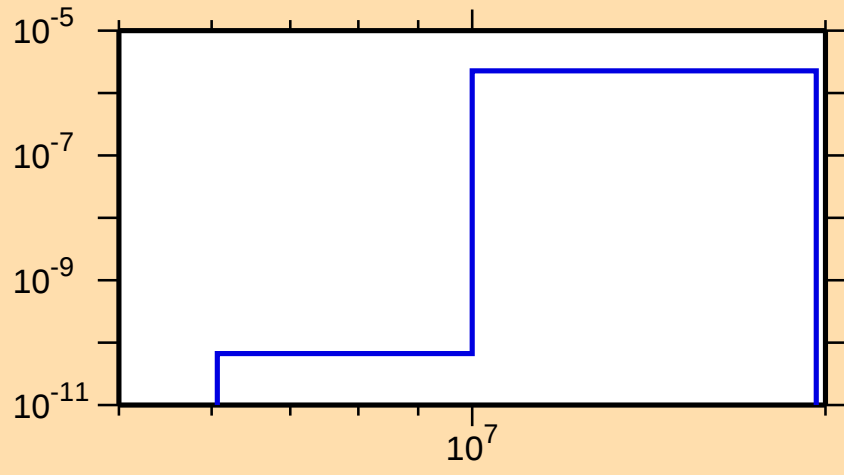
\sigma vs. E for ^{200}\text{Rn}(n,\text{He}3)
