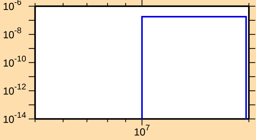
\sigma vs. E for ^{200}\text{Rn}(n,2n\alpha)
