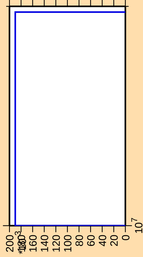
\Delta\sigma/\sigma vs. E for ^{200}\text{Rn}(n,nt)
