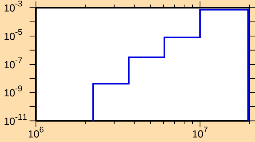
\sigma vs. E for ^{200}\text{Rn}(n,n\alpha)
