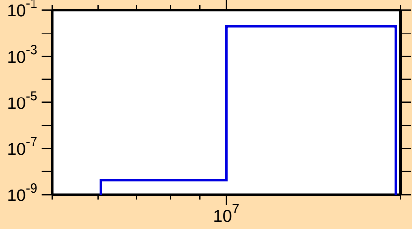
\sigma vs. E for ^{204}\text{Rn}(n,2n)
