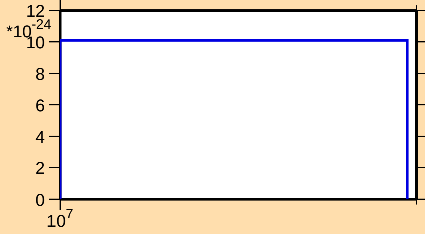
\sigma vs. E for ^{204}\text{Rn}(\text{mt 11})
