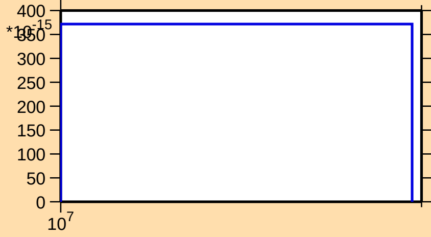
\sigma vs. E for ^{204}\text{Rn}(n,\text{pt})
