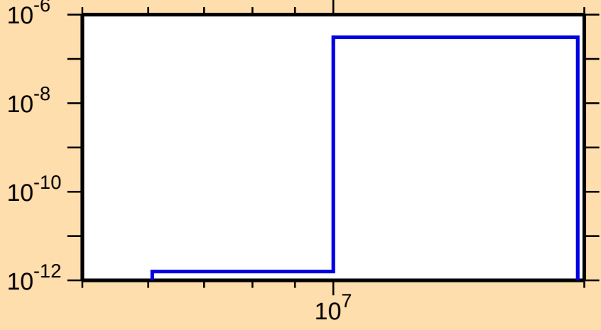
\sigma vs. E for ^{204}\text{Rn}(n,\text{He3})
