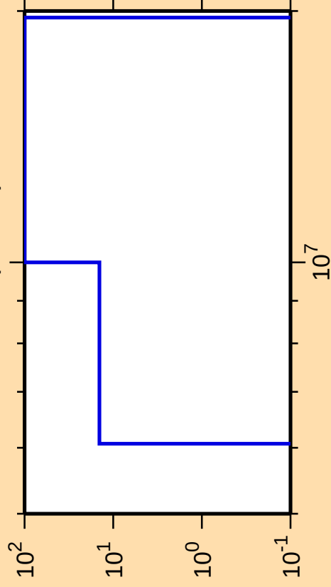
\Delta\sigma/\sigma vs. E for ^{204}\text{Rn}(n,\text{He3})
