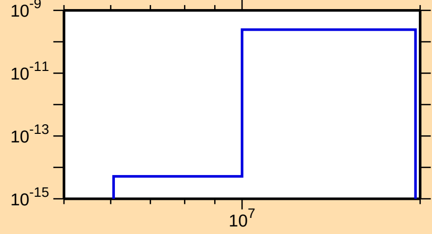
\sigma vs. E for ^{204}\text{Rn}(\text{mt } 45)
