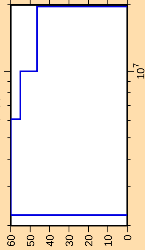
\Delta\sigma/\sigma vs. E for ^{204}\text{Rn}(n,p)
