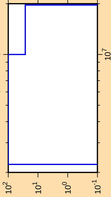
\Delta\sigma/\sigma vs. E for ^{204}\text{Rn}(n,n\text{cont.})
