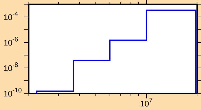
\sigma vs. E for ^{204}\text{Rn}(n,\alpha)
