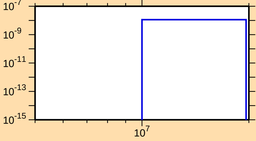
\sigma vs. E for ^{204}\text{Rn}(n,2n\alpha)
