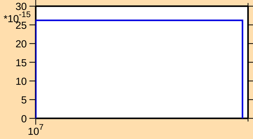
\sigma vs. E for ^{204}\text{Rn}(\text{mt } 34)
