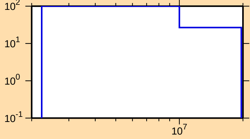
\Delta\sigma/\sigma vs. E for ^{204}\text{Rn}(n,n\text{cont.})
