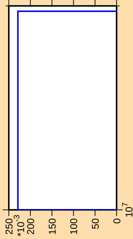
\Delta\sigma/\sigma vs. E for ^{204}\text{Rn}(\text{mt } 34)
