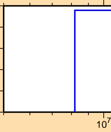
\sigma vs. E for ^{204}\text{Rn}(\text{mt } 34)
