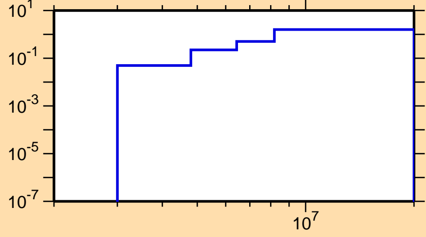
\sigma vs. E for ^{204}\text{Rn}(n,n\text{cont.})
