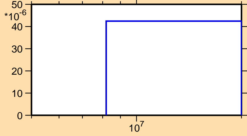
\sigma vs. E for ^{204}\text{Rn}(n,t)
