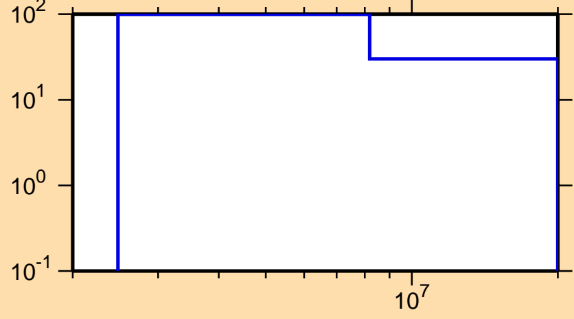
\Delta\sigma/\sigma vs. E for ^{204}\text{Rn}(n,ncont.)
