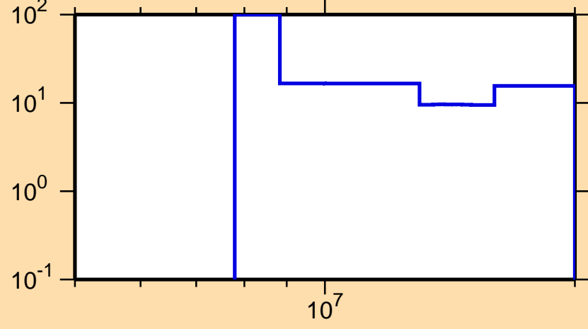
\Delta\sigma/\sigma vs. E for ^{210}\text{Rn}(n,2n)
