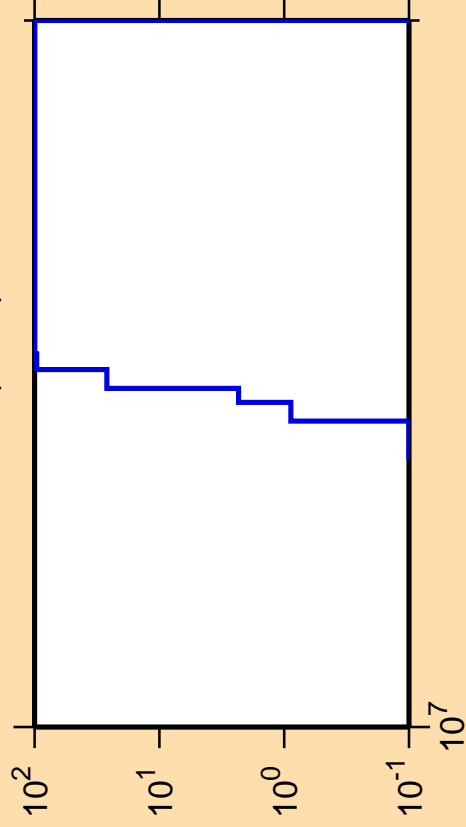
\Delta\sigma/\sigma vs. E for ^{210}\text{Rn}(n,nd)
