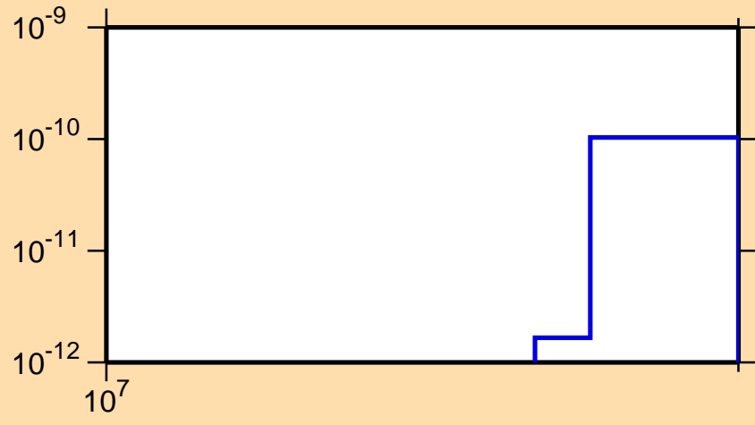
\sigma vs. E for ^{210}\text{Rn}(n,\text{pt})
