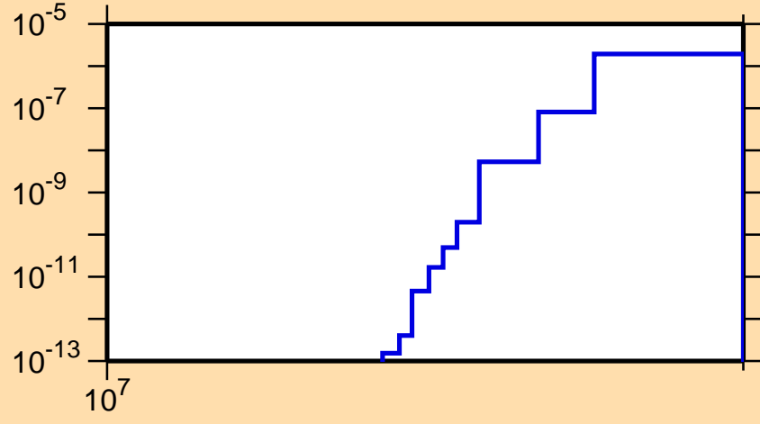
\sigma vs. E for ^{210}\text{Rn}(n,nd)
