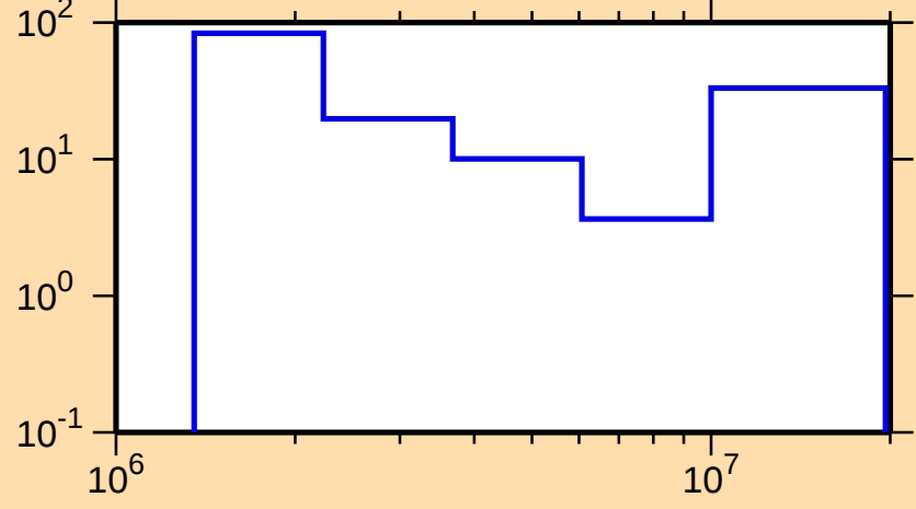
\Delta\sigma/\sigma vs. E for ^{210}\text{Rn}(n,n\text{cont.})
