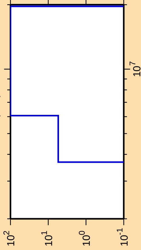
\Delta\sigma/\sigma vs. E for ^{210}\text{Rn}(n,d)
