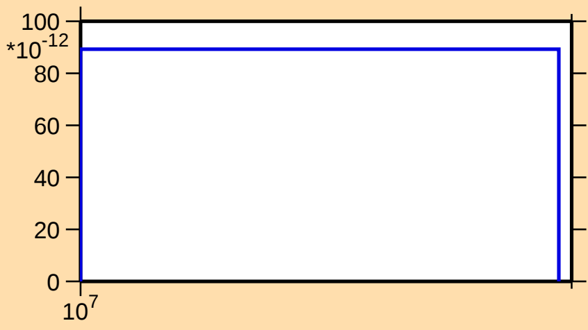
\sigma vs. E for ^{210}\text{Rn}(\text{mt117})
