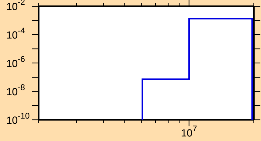
\sigma vs. E for ^{210}\text{Rn}(n,d)
