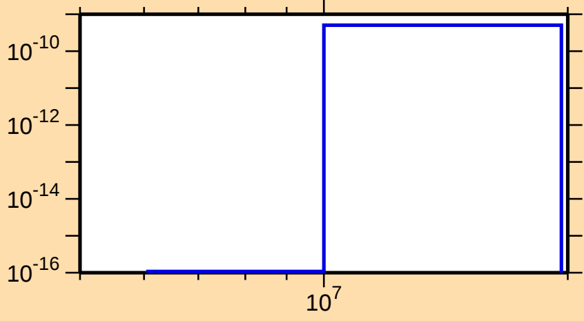
\sigma vs. E for ^{210}\text{Rn}(\text{mt } 45)
