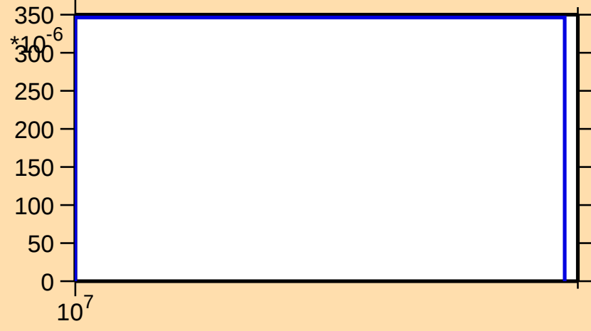
\sigma vs. E for ^{210}\text{Rn}(n,3n)
