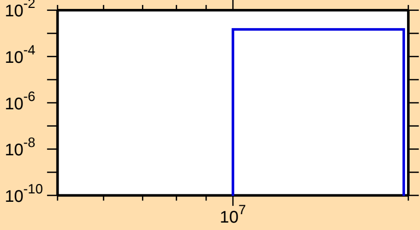
\sigma vs. E for ^{210}\text{Rn}(n,2n\alpha)
