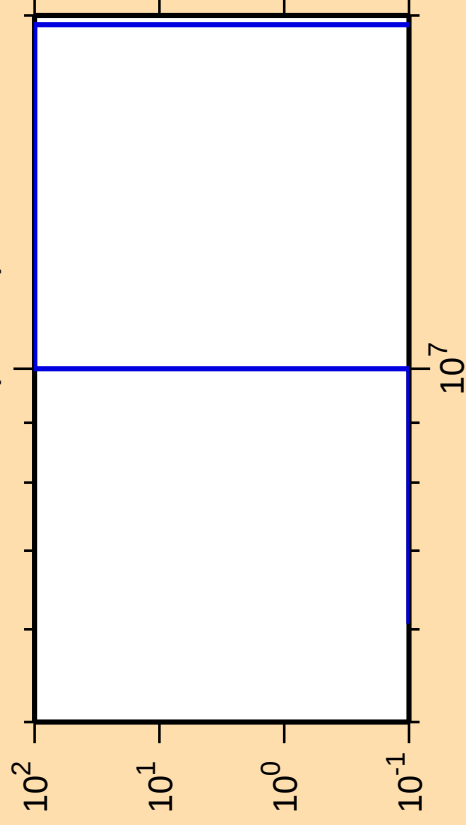
\Delta\sigma/\sigma vs. E for ^{210}\text{Rn}(\text{mt } 45)
