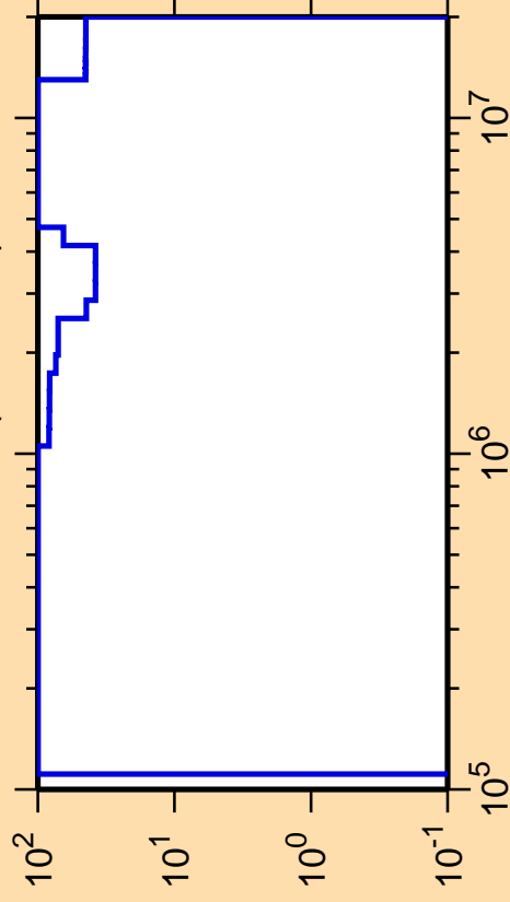
\Delta\sigma/\sigma vs. E for ^{225}\text{Rn}(n,\text{ncont.})
