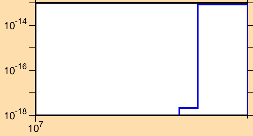
\sigma vs. E for ^{225}\text{Rn}(n,\text{He}3)
