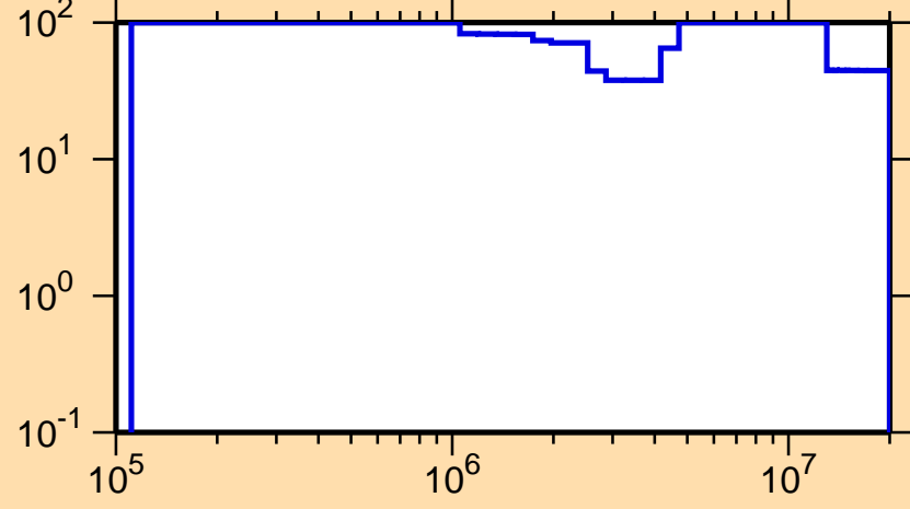
\Delta\sigma/\sigma vs. E for ^{225}\text{Rn}(n,n\text{cont.})
