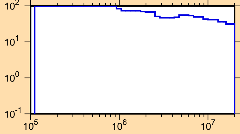
\Delta\sigma/\sigma vs. E for ^{225}\text{Rn}(n,\text{nonel.})
