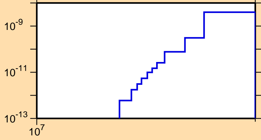
\sigma vs. E for ^{225}\text{Rn}(n,3n\alpha)
