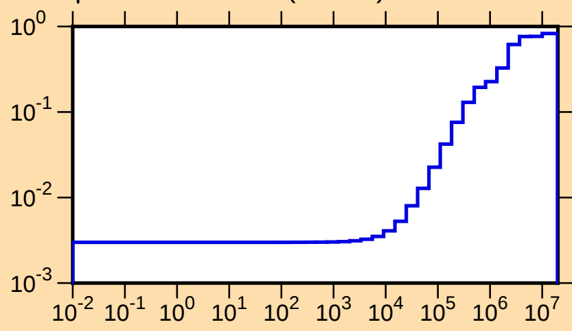
\mu vs. E for ^{225}\text{Rn}(\text{mt251})
