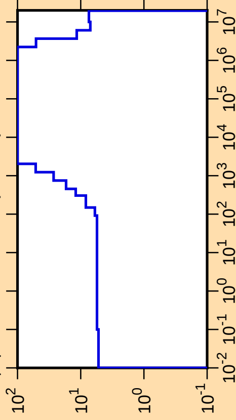
\Delta\mu/\mu vs. E for ^{225}\text{Rn}(\text{mt251})
