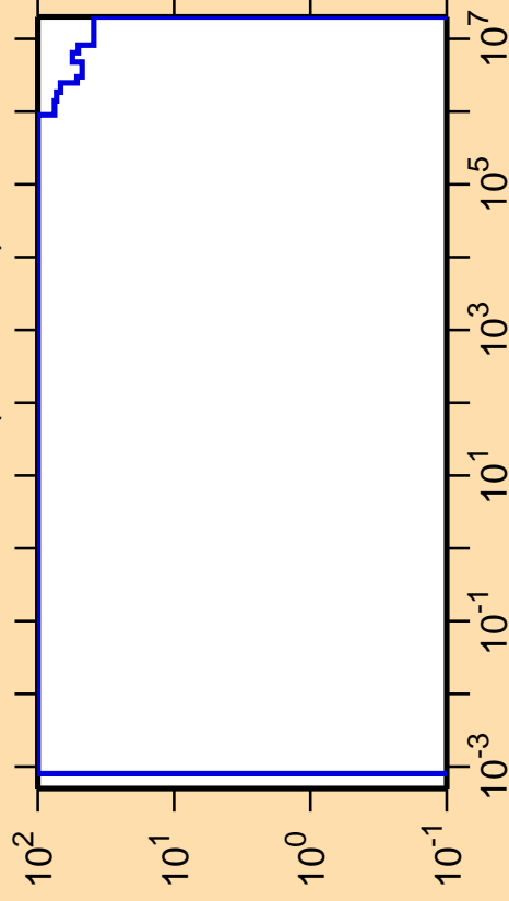
\Delta\sigma/\sigma vs. E for ^{225}\text{Rn}(n,\text{nonel.})
