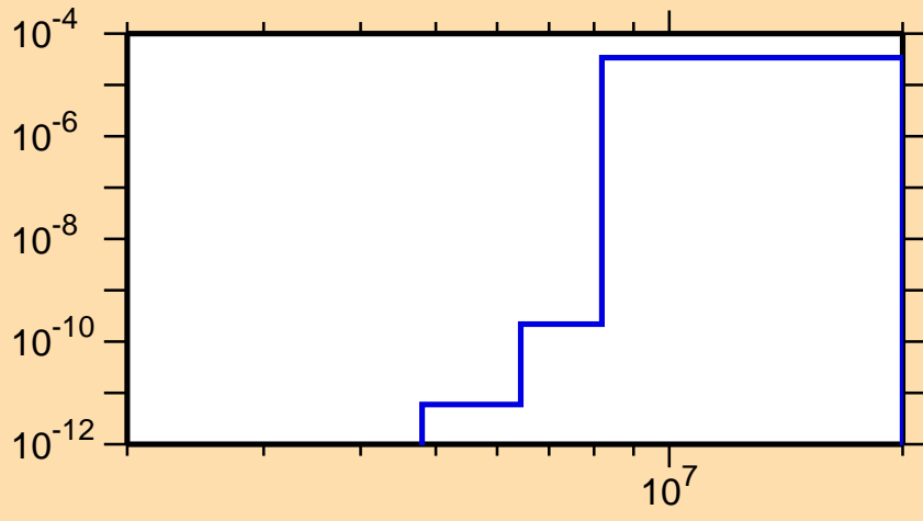
\sigma vs. E for ^{225}\text{Rn}(n,n\alpha)
