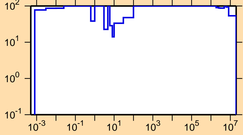
\Delta\sigma/\sigma vs. E for ^{225}\text{Rn}(n,\text{tot.})
