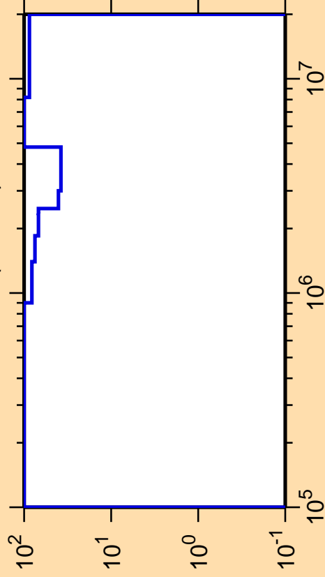
\Delta\sigma/\sigma vs. E for ^{225}\text{Rn}(n,\text{inel.})
