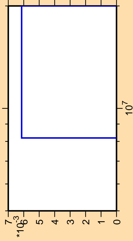
\Delta\sigma/\sigma vs. E for ^{225}\text{Rn}(n,\text{He}3)
