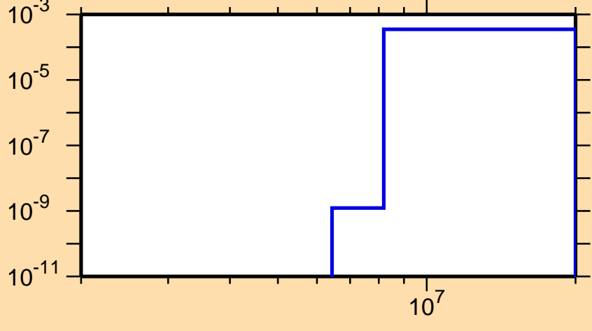
\sigma vs. E for ^{225}\text{Rn}(n,p)
