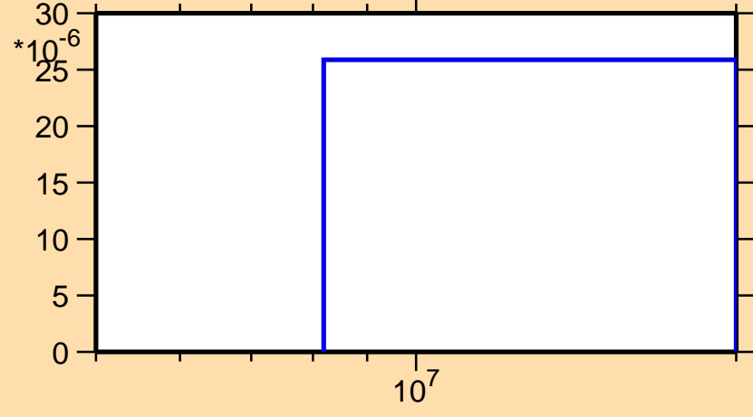
\sigma vs. E for ^{225}\text{Rn}(n,t)
