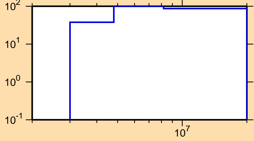
\Delta\sigma/\sigma vs. E for ^{225}\text{Rn}(n,\text{inel.})
