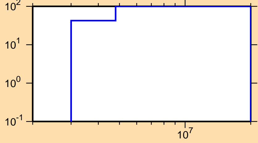
\Delta\sigma/\sigma vs. E for ^{225}\text{Rn}(n,ncont.)
