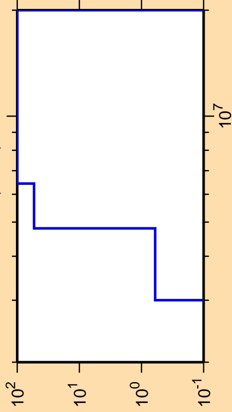
\Delta\sigma/\sigma vs. E for ^{225}\text{Rn}(n,n\alpha)
