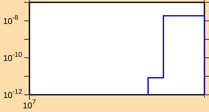
\sigma vs. E for ^{97}\text{Ru}(n,\text{pt})
