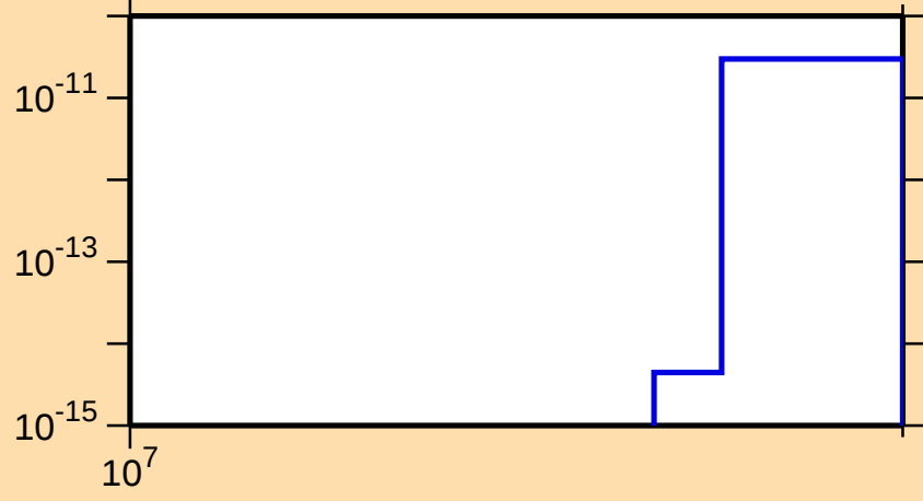
\sigma vs. E for ^{97}\text{Ru}(\text{mt } 34)
