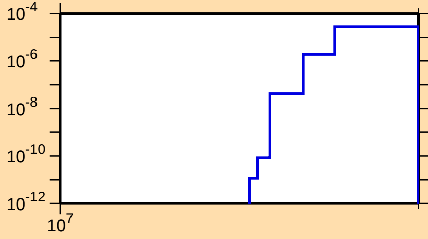
\sigma vs. E for ^{97}\text{Ru}(n,\text{nd})
