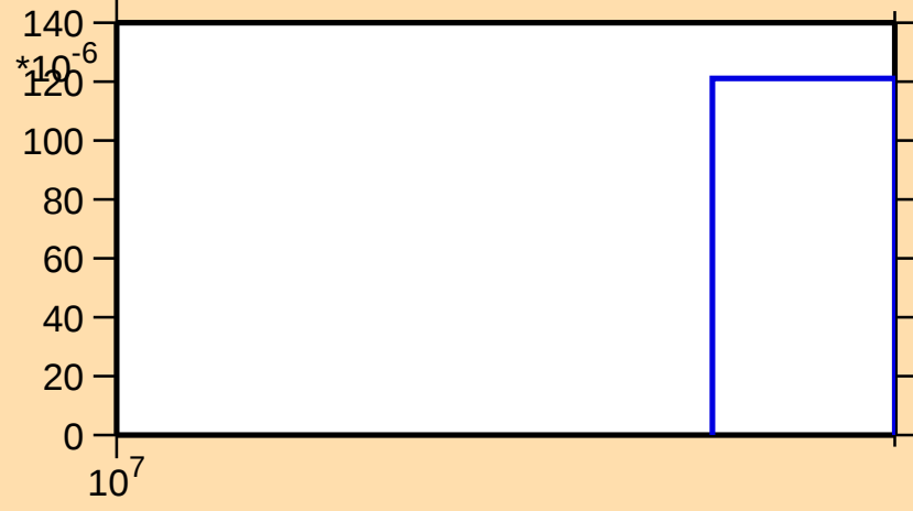
\sigma vs. E for ^{97}\text{Ru}(n,3n)
