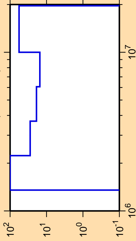
\Delta\sigma/\sigma vs. E for ^{97}\text{Ru}(n,ncont.)
