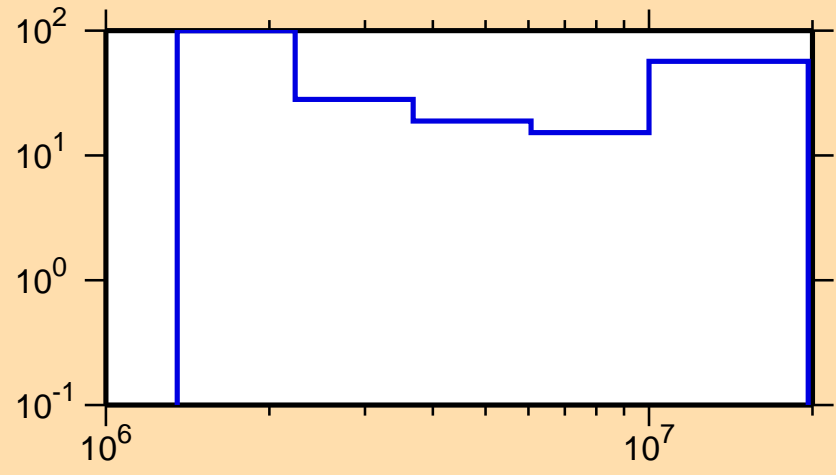
\Delta\sigma/\sigma vs. E for ^{97}\text{Ru}(n,ncont.)
