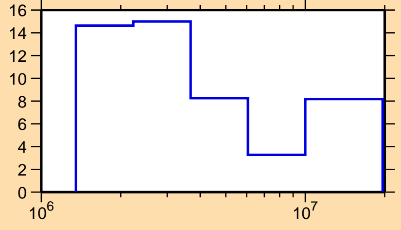
\Delta\sigma/\sigma vs. E for ^{97}\text{Ru}(n,tot.)
