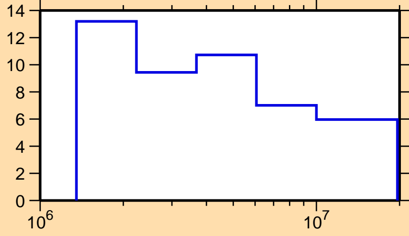
\Delta\sigma/\sigma vs. E for ^{97}\text{Ru}(n,n\text{nonel.})
