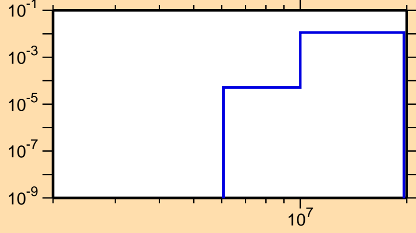
\sigma vs. E for ^{97}\text{Ru}(n,\alpha)
