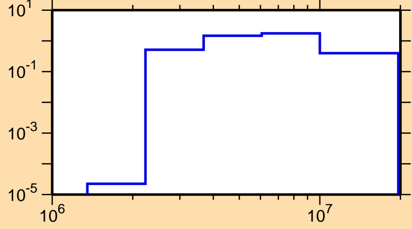
\sigma vs. E for ^{97}\text{Ru}(n,n\text{cont.})
