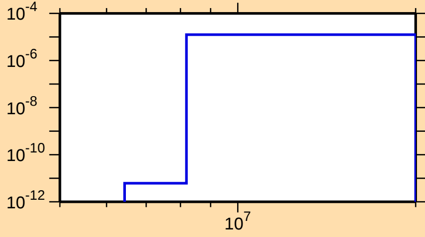
\sigma vs. E for ^{97}\text{Ru}(n,p\alpha)
