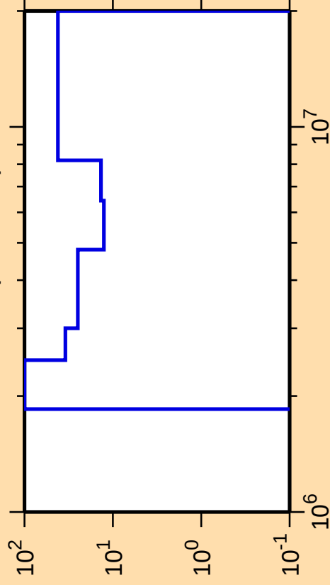
\Delta\sigma/\sigma vs. E for ^{97}\text{Ru}(n,\text{ncont.})
