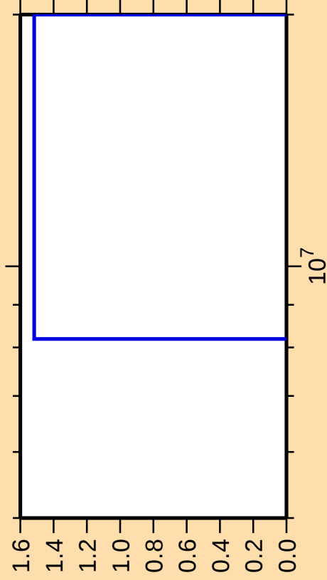
\Delta\sigma/\sigma vs. E for ^{97}\text{Ru}(\text{mt } 34)
