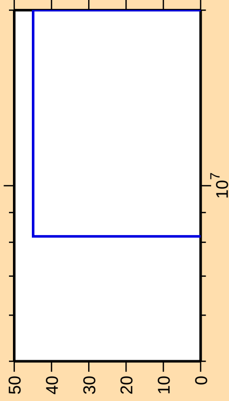
\Delta\sigma/\sigma vs. E for ^{97}\text{Ru}(\text{mt } 45)
