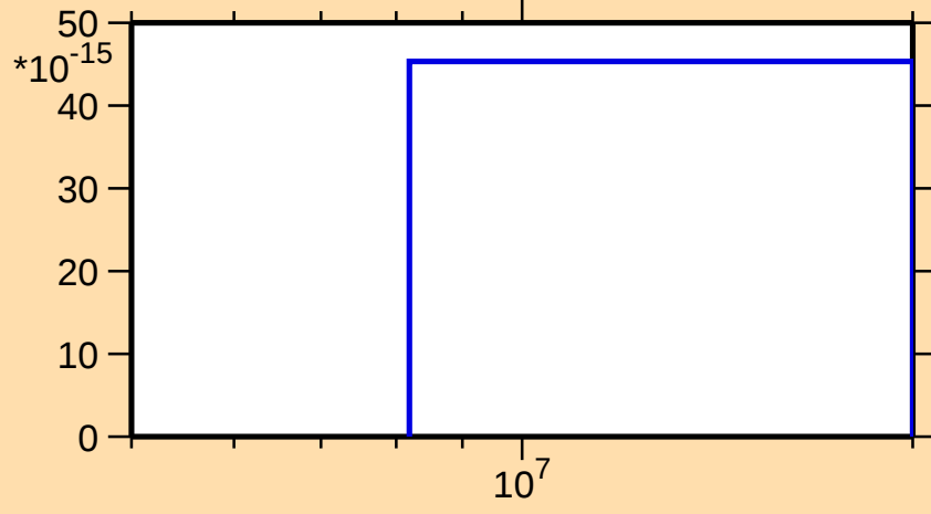
\sigma vs. E for ^{102}\text{Ru}(n,2np)
