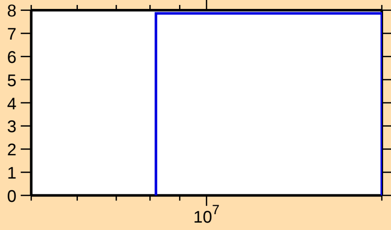
\Delta\sigma/\sigma vs. E for ^{102}\text{Ru}(n,\text{el.})
