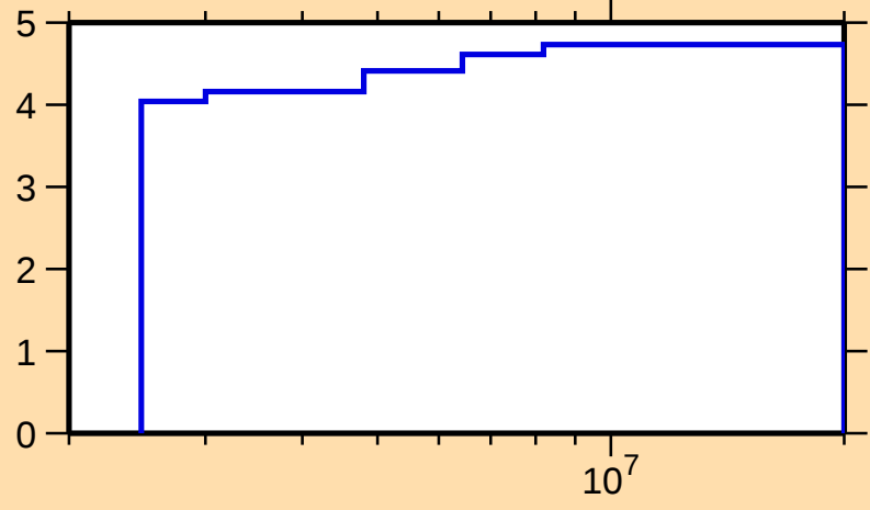
\Delta\sigma/\sigma vs. E for ^{102}\text{Ru}(\text{n},\text{nonel.})
