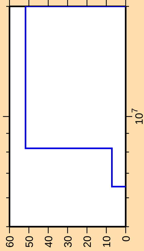
\Delta\sigma/\sigma vs. E for ^{102}\text{Ru}(n,n\alpha)
