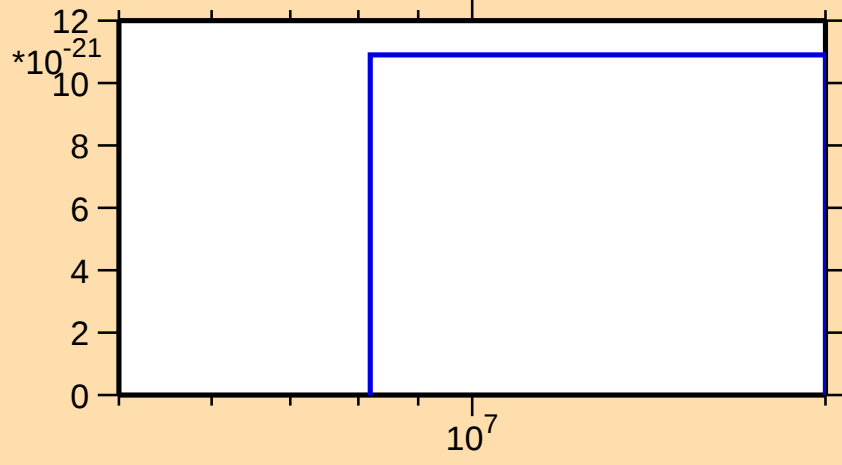
\sigma vs. E for ^{102}\text{Ru}(\text{mt } 34)
