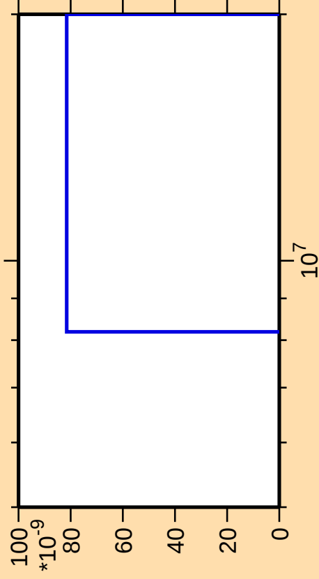
\Delta\sigma/\sigma vs. E for ^{102}\text{Ru}(\text{mt } 34)
