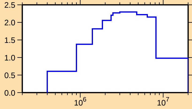
\sigma vs. E for ^{102}\text{Ru}(\text{n,inel.})
