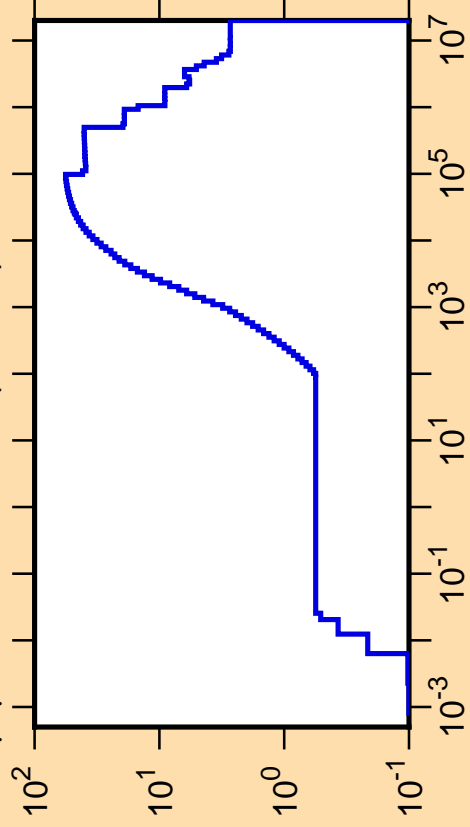
\Delta\mu/\mu vs. E for ^{104}\text{Ru}(\text{mt251})
