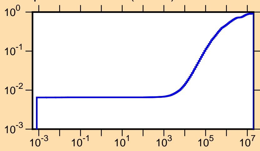
\mu vs. E for ^{104}\text{Ru}(\text{mt251})
