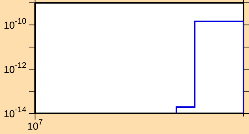
\sigma vs. E for ^{104}\text{Ru}(n,nt)
