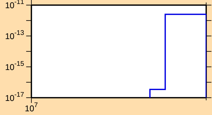
\sigma vs. E for ^{104}\text{Ru}(n,\text{He3})
