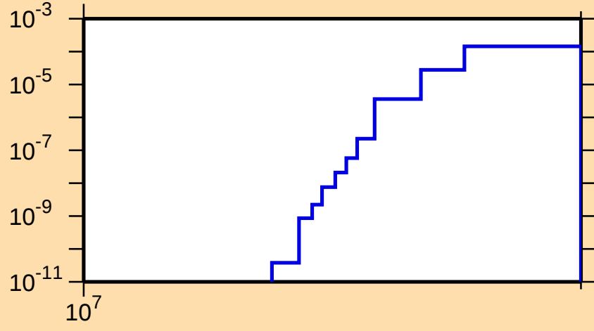
\sigma vs. E for ^{104}\text{Ru}(n,t)
