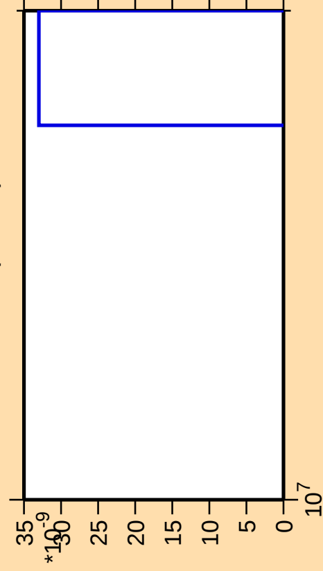
\Delta\sigma/\sigma vs. E for ^{104}\text{Ru}(n,3n\alpha)
