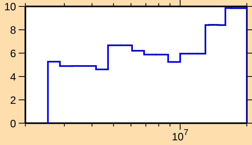
\Delta\sigma/\sigma vs. E for ^{104}\text{Ru}(\text{n,el.})
