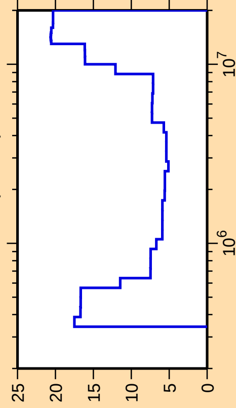
\Delta\sigma/\sigma vs. E for ^{104}\text{Ru}(\text{n,inel.})
