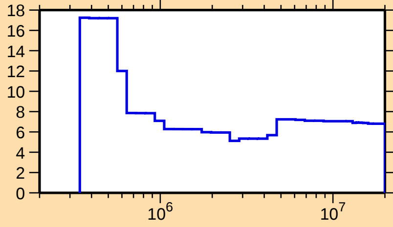
\Delta\sigma/\sigma vs. E for ^{104}\text{Ru}(\text{n,nonel.})
