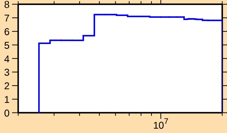
\Delta\sigma/\sigma vs. E for ^{104}\text{Ru}(\text{n},\text{nonel.})
