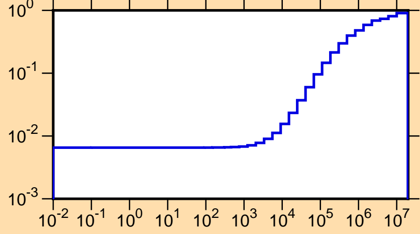
\mu vs. E for ^{104}\text{Ru}(\text{mt251})
