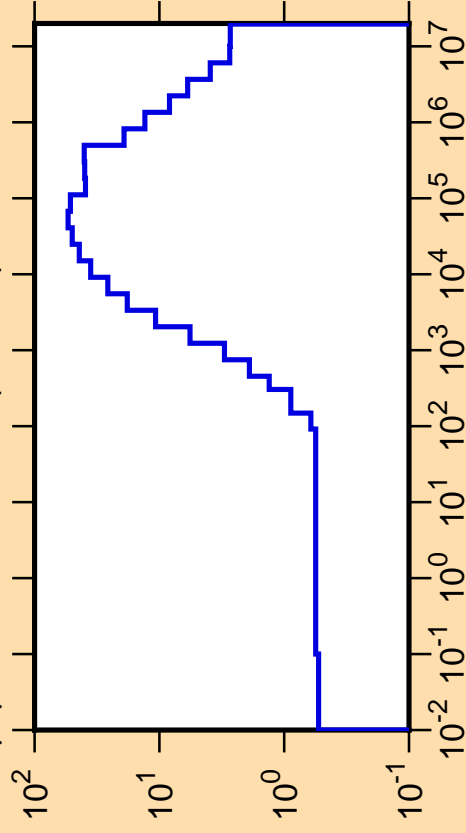
\Delta\mu/\mu vs. E for ^{104}\text{Ru}(\text{mt251})
