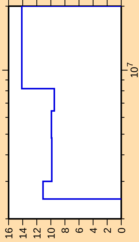
\Delta\sigma/\sigma vs. E for ^{104}\text{Ru}(\text{n,ncont.})
