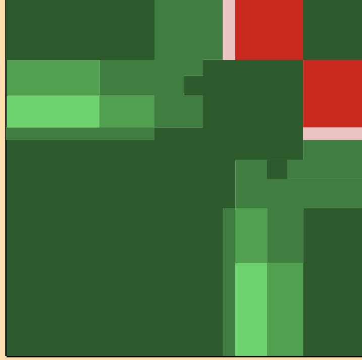
\sigma vs. E for ^{104}\text{Ru}(n,\text{inel.})
