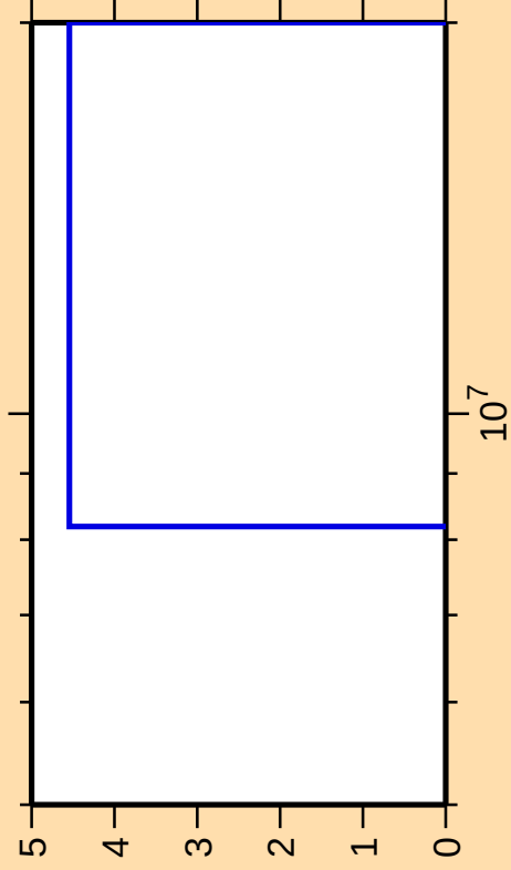
\Delta\sigma/\sigma vs. E for ^{104}\text{Ru}(n,\text{nd})
