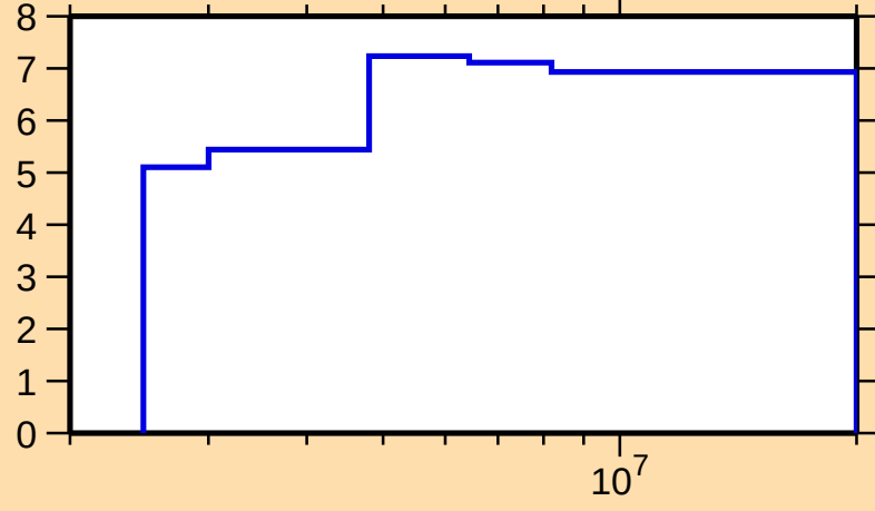
\Delta\sigma/\sigma vs. E for ^{104}\text{Ru}(\text{n,nonel.})
