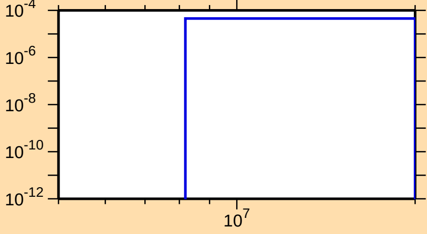
\sigma vs. E for ^{104}\text{Ru}(n,n\alpha)
