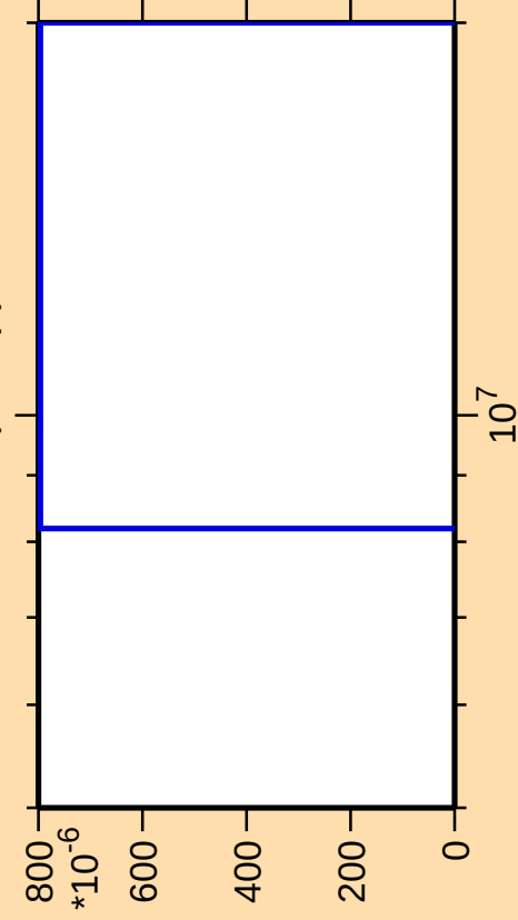
\Delta\sigma/\sigma vs. E for ^{104}\text{Ru}(n,2np)
