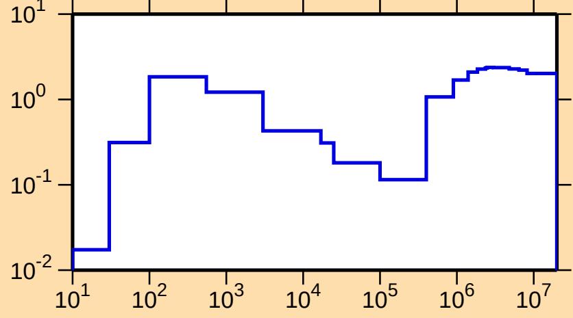
\sigma vs. E for ^{104}\text{Ru}(n,\text{nonel.})
