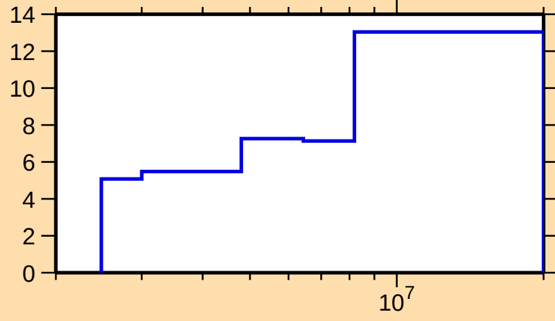
\Delta\sigma/\sigma vs. E for ^{104}\text{Ru}(\text{n,inel.})
