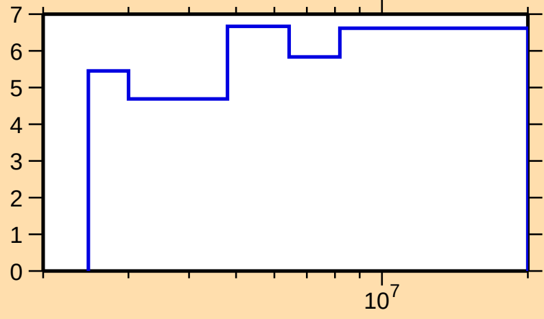
\Delta\sigma/\sigma vs. E for ^{104}\text{Ru}(\text{n,el.})
