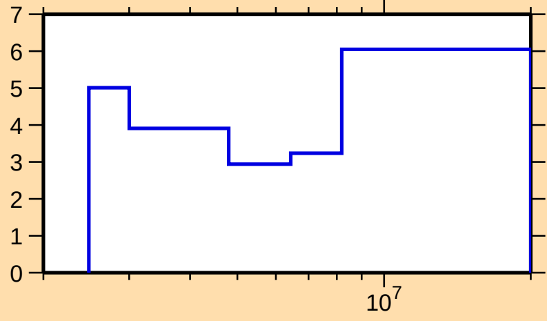
\Delta\sigma/\sigma vs. E for ^{104}\text{Ru}(\text{n},\text{tot.})
