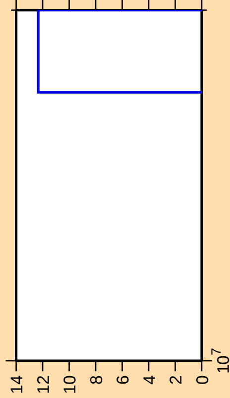
\Delta\sigma/\sigma vs. E for ^{34}\text{S}(\text{n},\text{pd})
