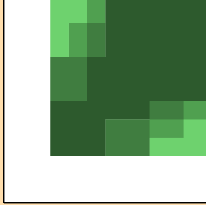
\sigma vs. E for ^{34}\text{S}(\text{n,ncont.})
