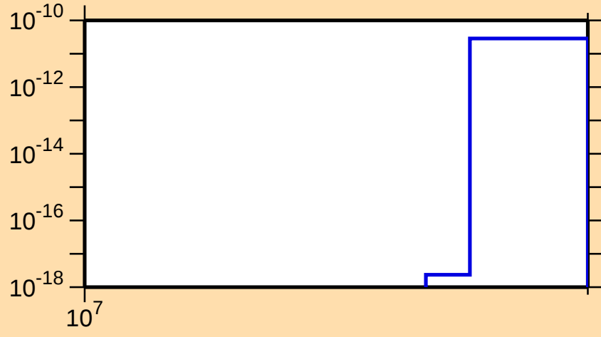
\sigma vs. E for ^{34}\text{S}(n,p\alpha)
