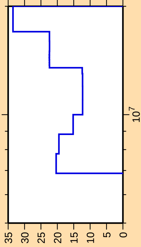
\Delta\sigma/\sigma vs. E for ^{34}\text{S}(\text{n,ncont.})
