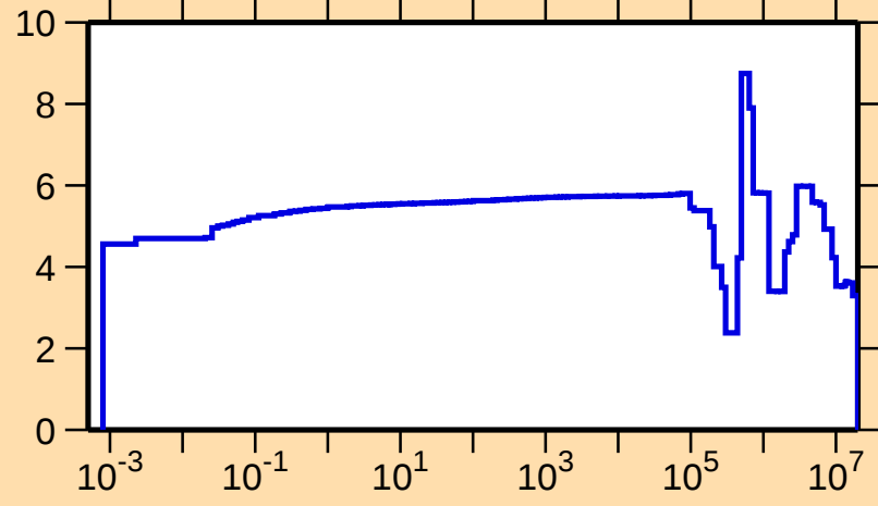
\Delta\sigma/\sigma vs. E for ^{34}\text{S}(\text{n,tot.})
