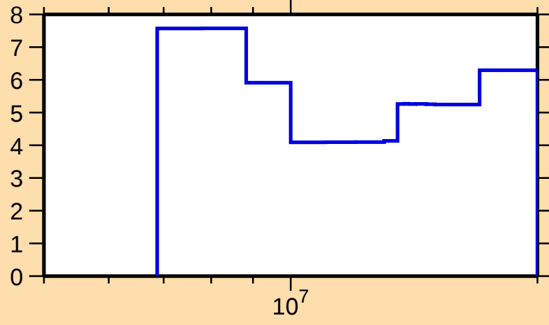
\Delta\sigma/\sigma vs. E for ^{34}\text{S}(\text{n},\text{el.})
