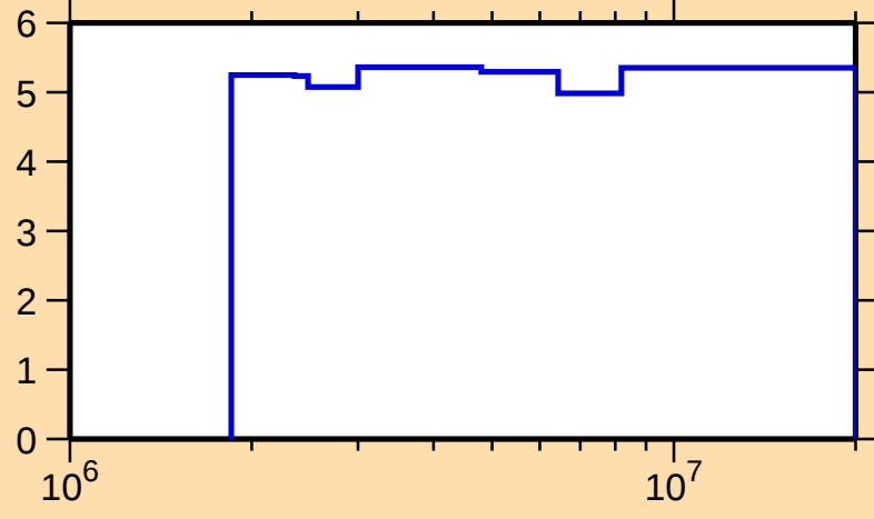
\Delta\sigma/\sigma vs. E for ^{34}\text{S}(\text{n,nonel.})
