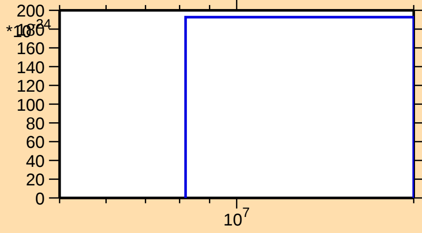
\sigma vs. E for ^{34}\text{S}(\text{mt117})
