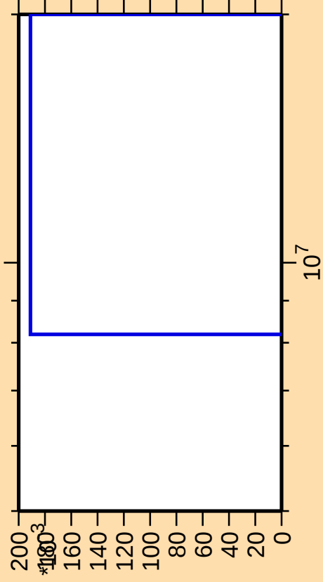
\Delta\sigma/\sigma vs. E for ^{34}\text{S}(n,p\alpha)
