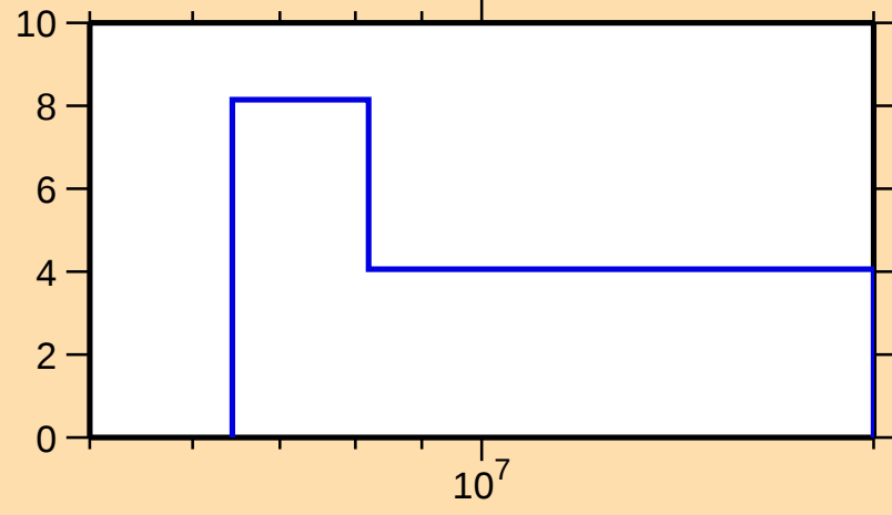
\Delta\sigma/\sigma vs. E for ^{34}\text{S}(\text{n},\text{el.})
