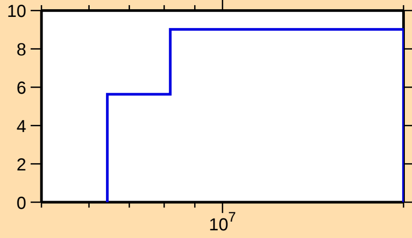
\Delta\sigma/\sigma vs. E for ^{34}\text{S}(\text{n},\text{inel.})
