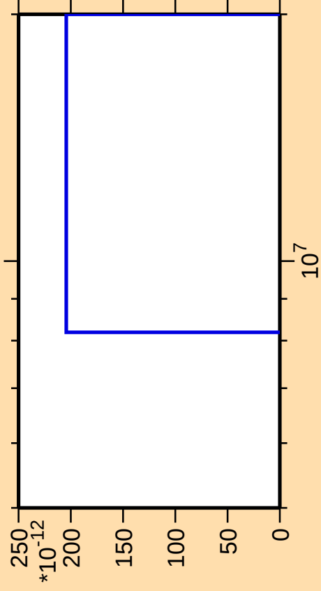
\Delta\sigma/\sigma vs. E for ^{34}\text{S}(\text{mt117})
