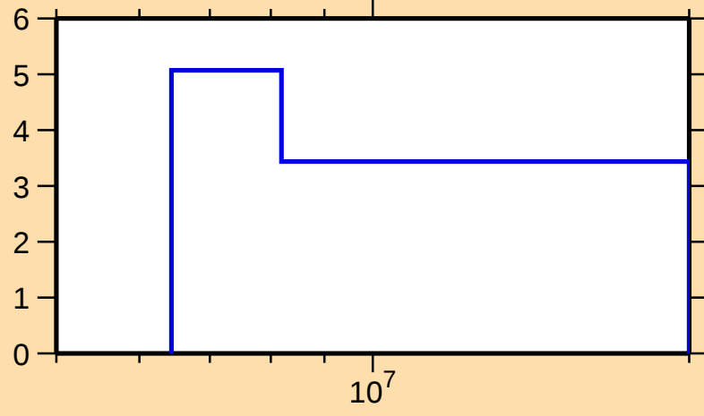
\Delta\sigma/\sigma vs. E for ^{34}\text{S}(\text{n},\text{tot.})
