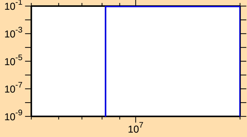
\sigma vs. E for ^{34}\text{S}(n,n\alpha)
