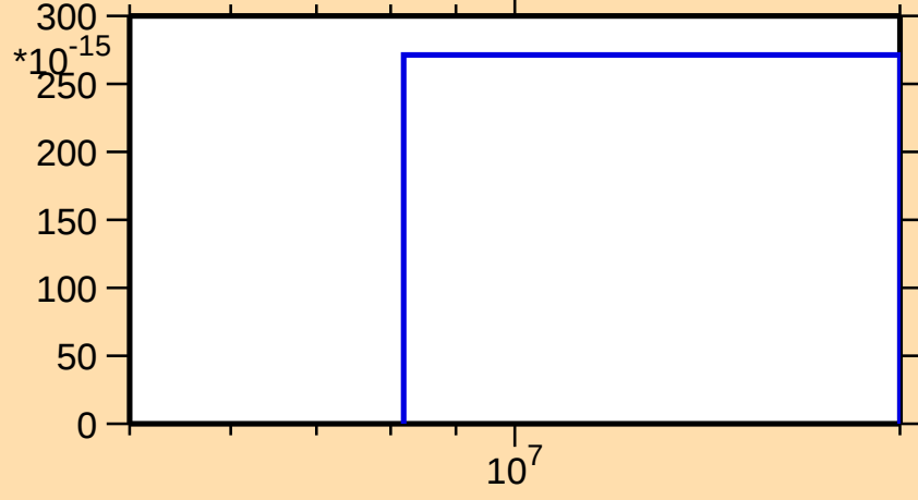
\sigma vs. E for ^{34}\text{S}(\text{n},\text{nd})
