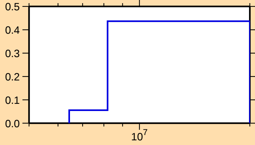
\sigma vs. E for ^{34}\text{S}(\text{n},\text{ncont.})
