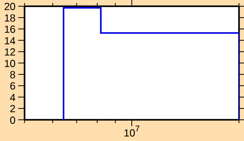
\Delta\sigma/\sigma vs. E for ^{34}\text{S}(n,n\text{cont.})
