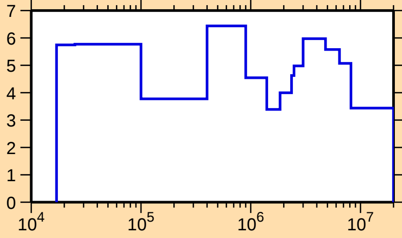
\Delta\sigma/\sigma vs. E for ^{34}\text{S}(\text{n,tot.})
