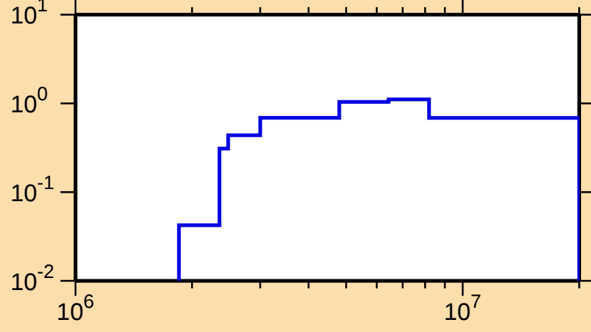
\sigma vs. E for ^{34}\text{S}(\text{n,inel.})
