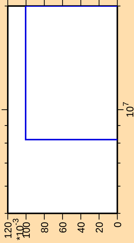
\Delta\sigma/\sigma vs. E for ^{34}\text{S}(\text{n},\text{pd})
