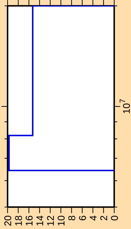
\Delta\sigma/\sigma vs. E for ^{34}\text{S}(\text{n},\text{ncont.})
