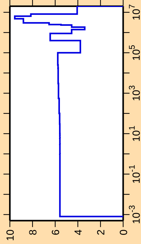
\Delta\sigma/\sigma vs. E for ^{34}\text{S}(\text{n,el.})
