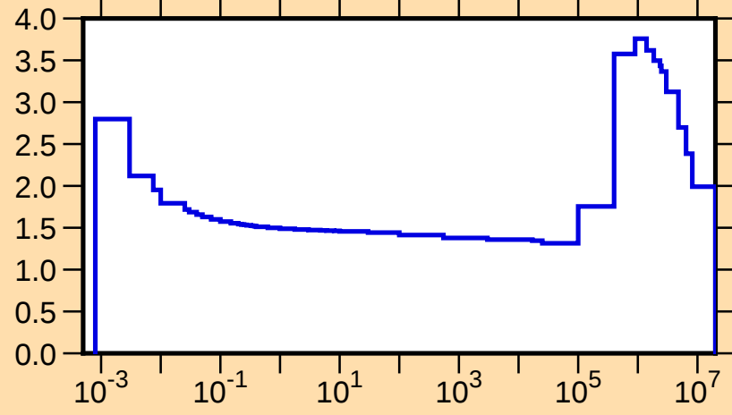
\sigma vs. E for ^{34}\text{S}(\text{n,tot.})
