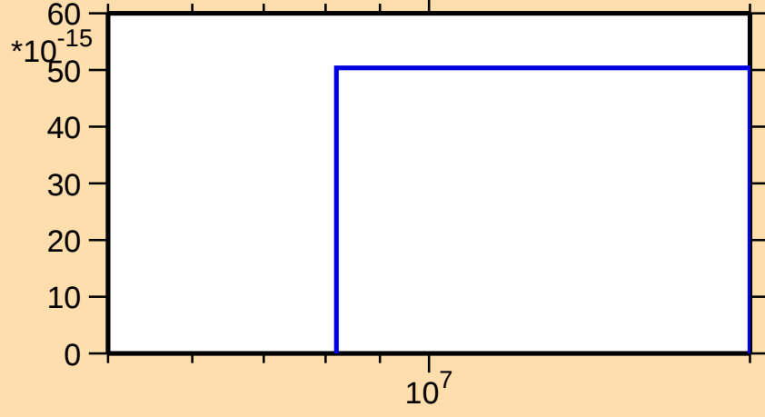
\sigma vs. E for ^{34}\text{S}(\text{n},\text{pd})
