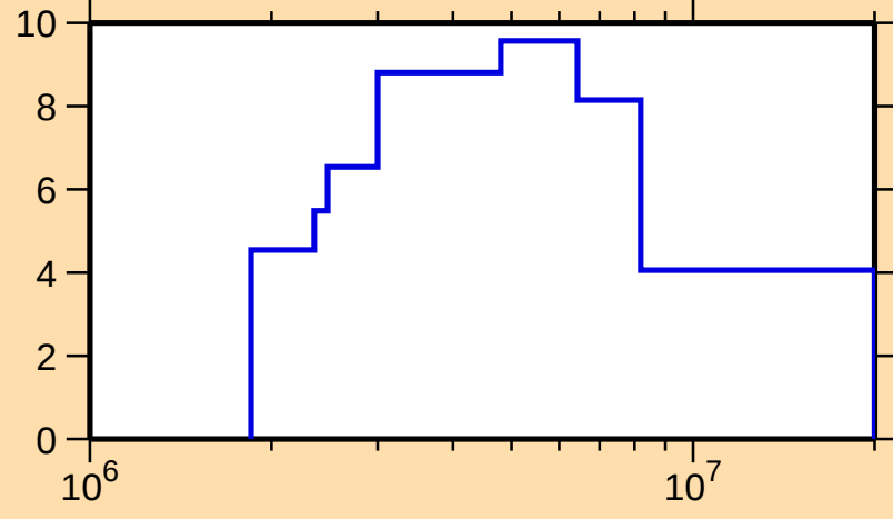
\Delta\sigma/\sigma vs. E for ^{34}\text{S}(\text{n,el.})
