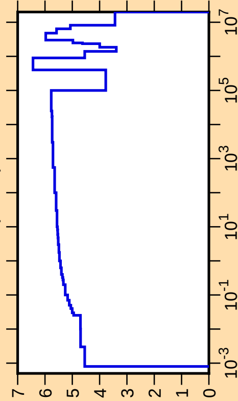
\Delta\sigma/\sigma vs. E for ^{34}\text{S}(\text{n,tot.})
