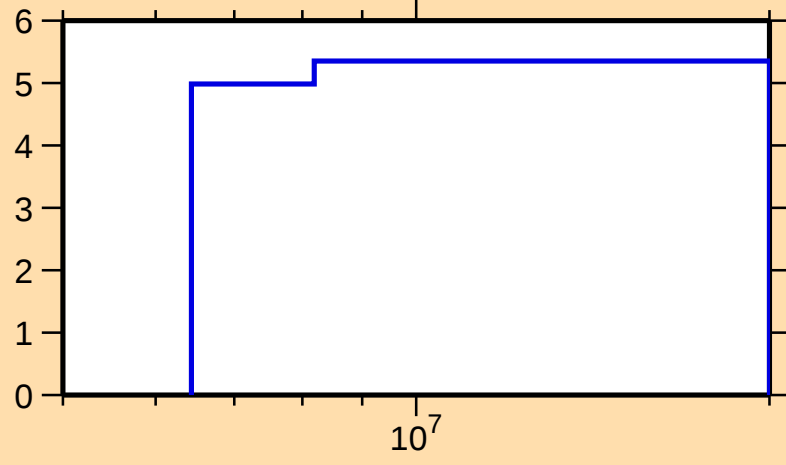
\Delta\sigma/\sigma vs. E for ^{34}\text{S}(\text{n},\text{nonel.})
